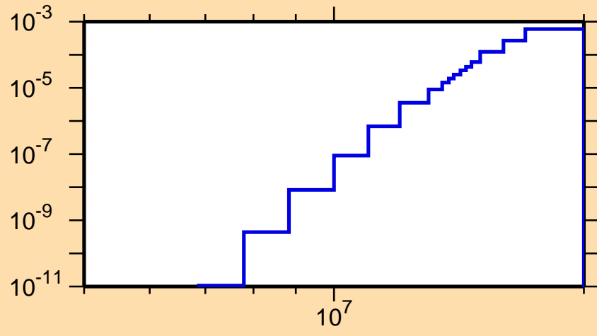
\sigma vs. E for ^{126}\text{La}(n,\text{He3})
