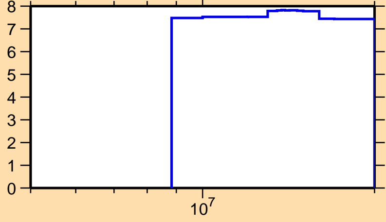
\Delta\sigma/\sigma vs. E for ^{126}\text{La}(n,\text{nonel.})
