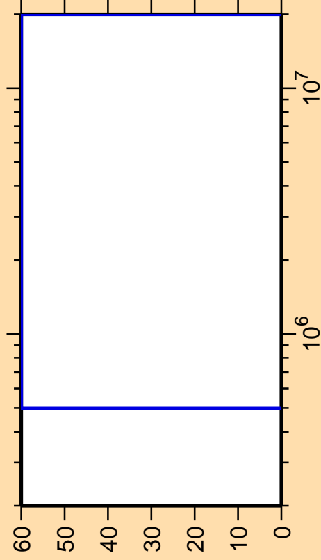
\Delta\sigma/\sigma vs. E for ^{126}\text{La}(n,\alpha)
