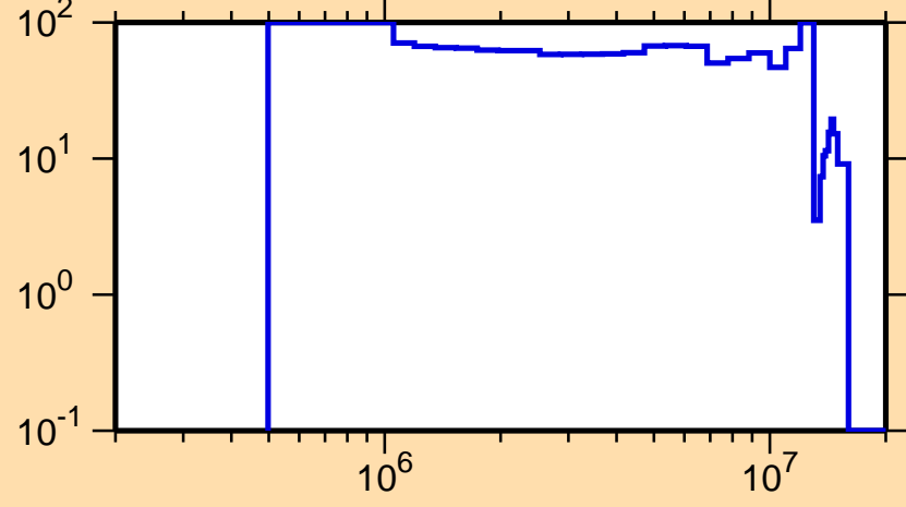
\Delta\sigma/\sigma vs. E for ^{126}\text{La}(n,n_1)
