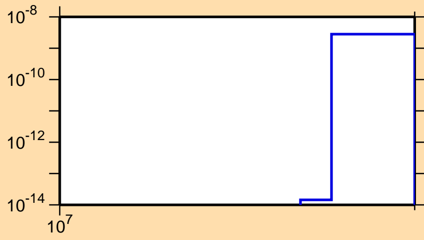
\sigma vs. E for ^{126}\text{La}(n,nt)
