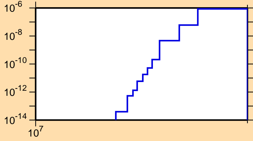
\sigma vs. E for ^{126}\text{La}(n,2n\alpha)
