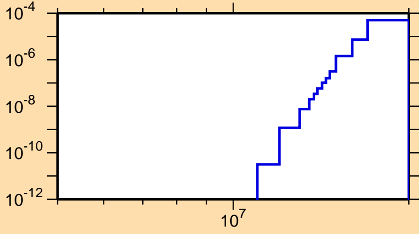
\sigma vs. E for ^{126}\text{La} (mt 45)
