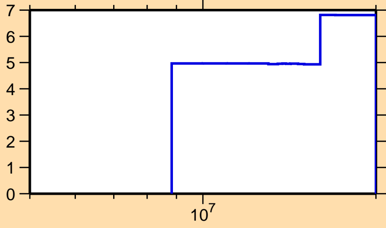
\Delta\sigma/\sigma vs. E for ^{126}\text{La}(n,\text{tot.})
