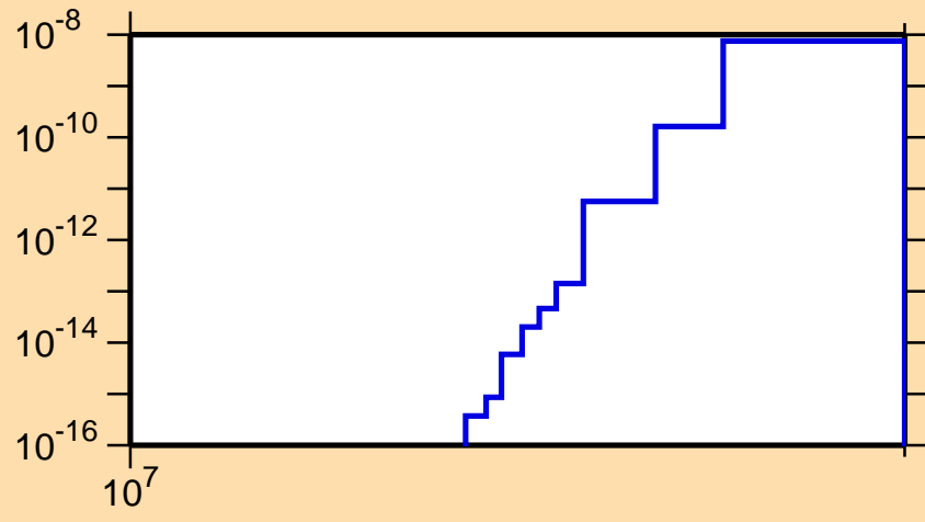
\sigma vs. E for ^{126}\text{La} (mt 34)
