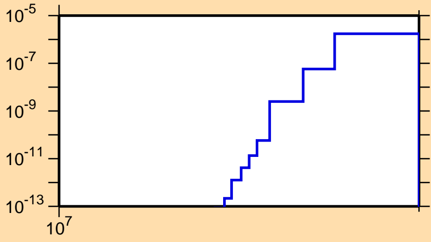
\sigma vs. E for ^{126}\text{La}(n,\text{pt})
