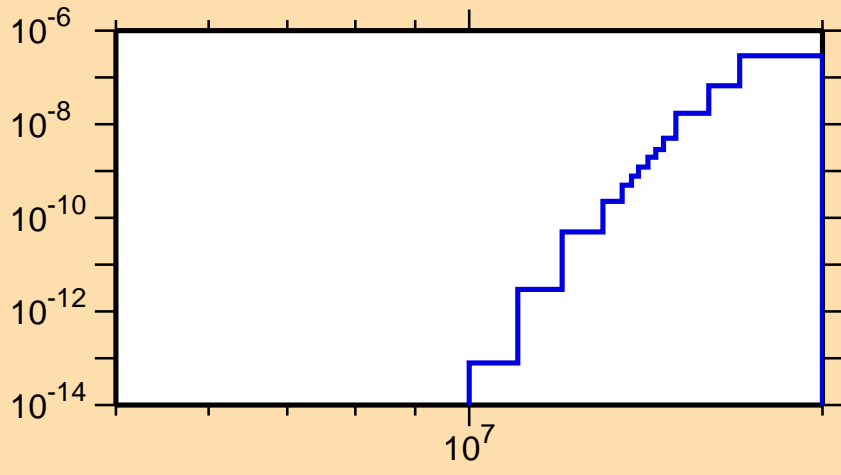
\sigma vs. E for ^{126}\text{La}(\text{mt117})
