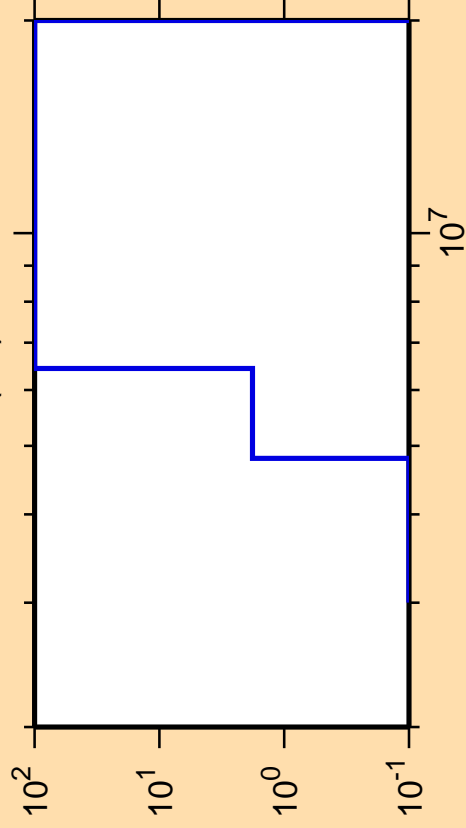
\Delta\sigma/\sigma vs. E for ^{126}\text{La}(n,t)
