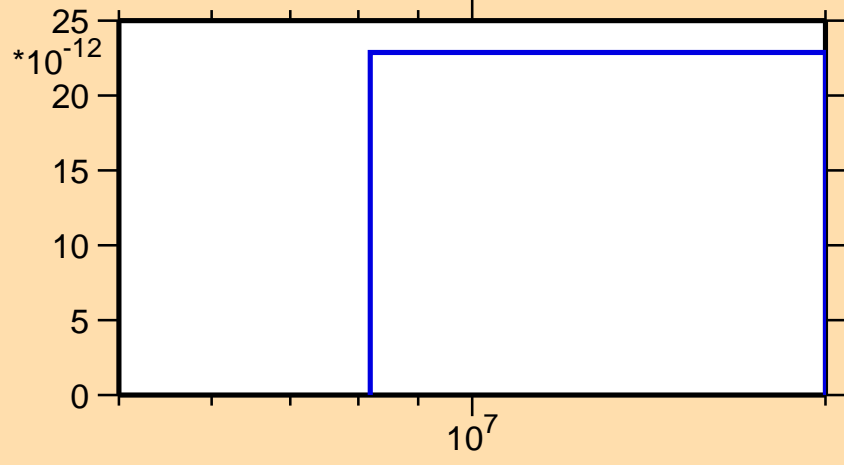
\sigma vs. E for ^{126}\text{La}(n,nt)
