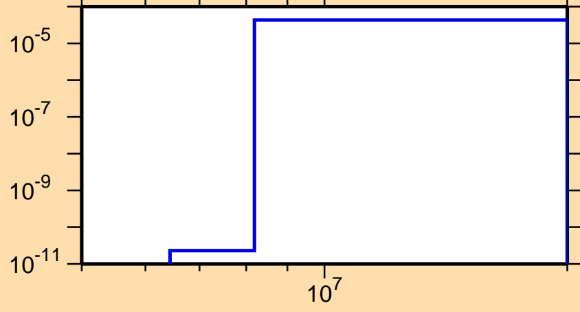
\sigma vs. E for ^{126}\text{La}(n,\text{He3})
