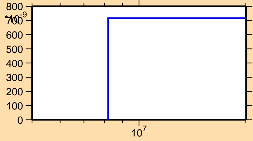
\sigma vs. E for ^{126}\text{La}(n,pd)
