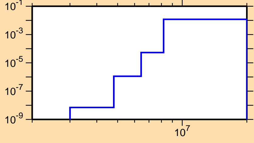
\sigma vs. E for ^{126}\text{La}(n,d)
