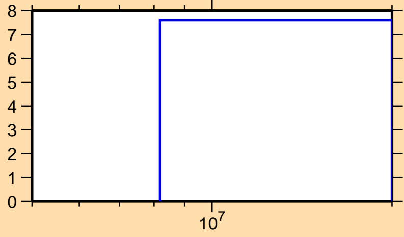
\Delta\sigma/\sigma vs. E for ^{126}\text{La}(n,\text{nonel.})
