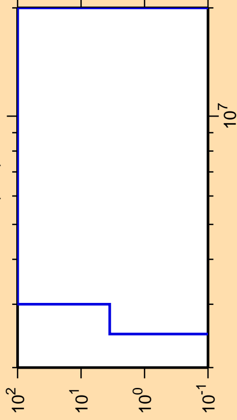
\Delta\sigma/\sigma vs. E for ^{126}\text{La}(n,d)
