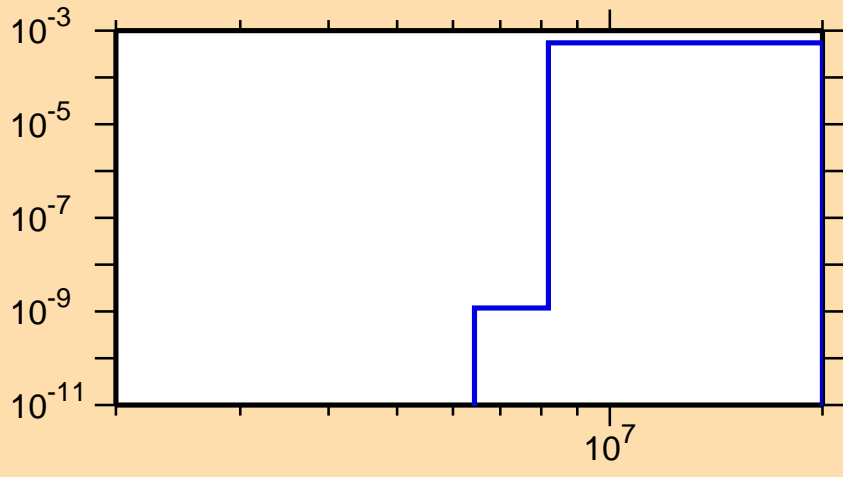
\sigma vs. E for ^{126}\text{La}(n,t)
