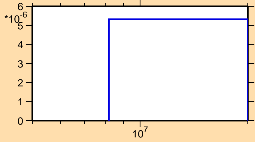
\sigma vs. E for ^{126}\text{La}(n,\text{nd})
