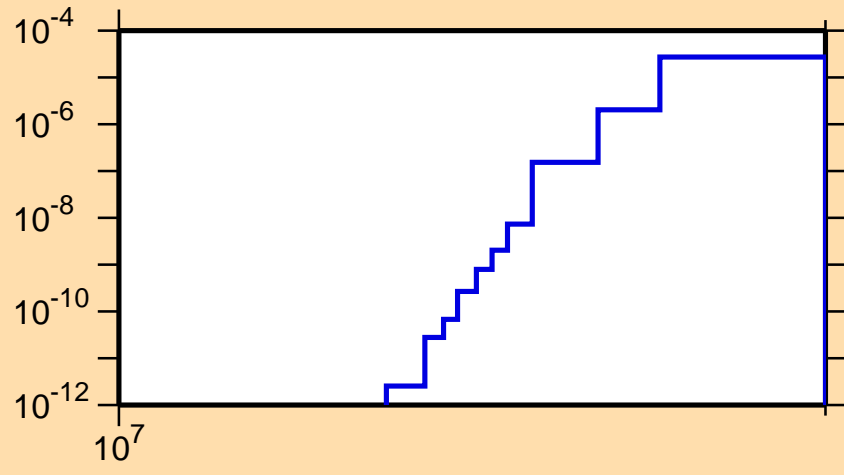
\sigma vs. E for ^{126}\text{La}(n,pt)
