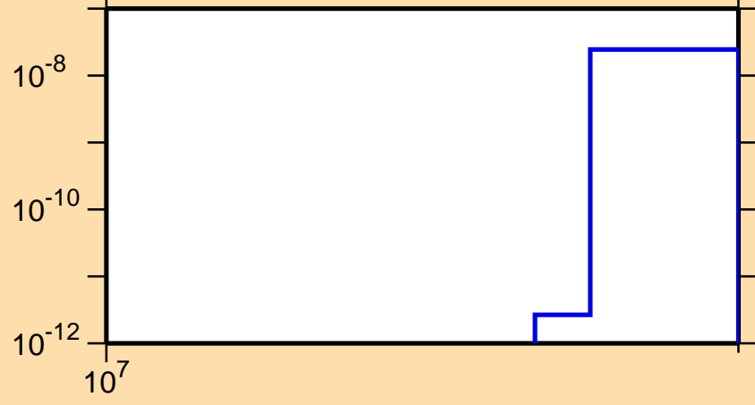
\sigma vs. E for ^{126}\text{La}(n,nt)
