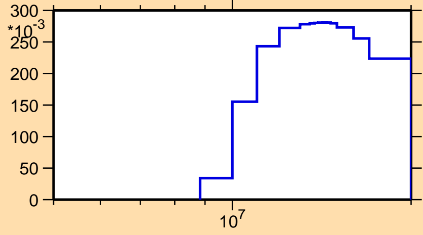
\sigma vs. E for ^{126}\text{La}(n,2n)
