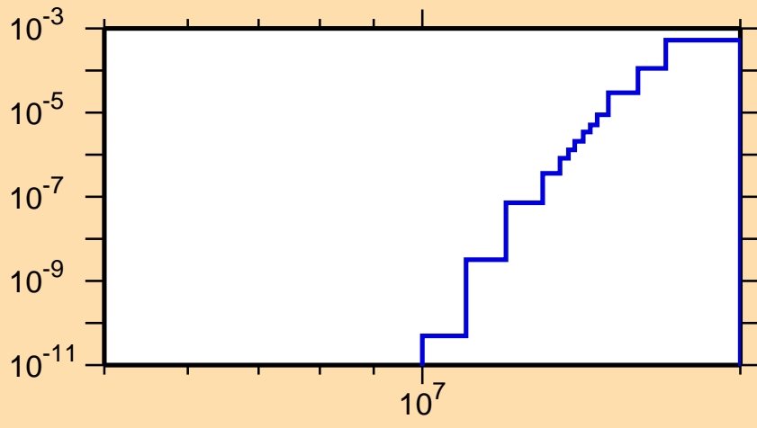
\sigma vs. E for ^{126}\text{La} (mt 45)
