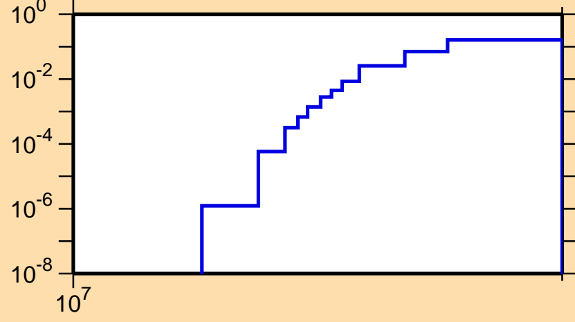
\sigma vs. E for ^{126}\text{La}(n,2np)
