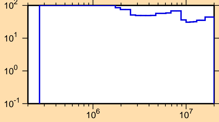
\Delta\sigma/\sigma vs. E for ^{126}\text{La}(n,n\text{cont.})
