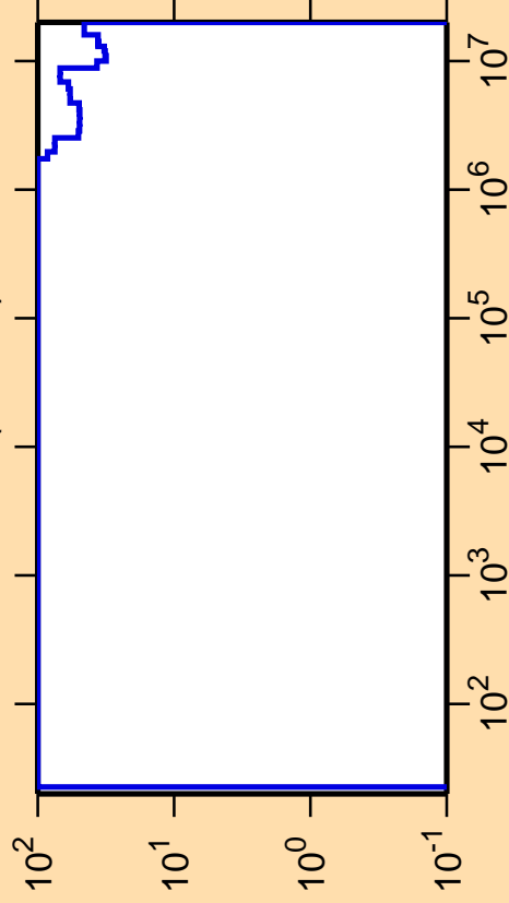
\Delta\sigma/\sigma vs. E for ^{126}\text{La}(n,\text{inel.})
