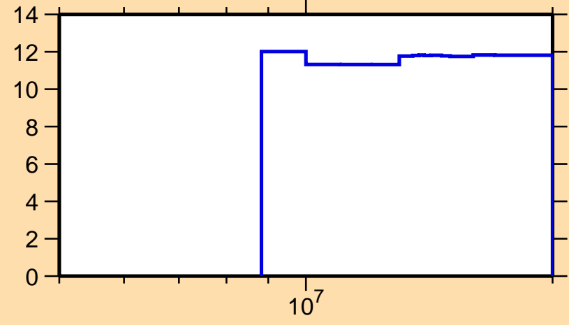
\Delta\sigma/\sigma vs. E for ^{126}\text{La}(n,\text{tot.})
