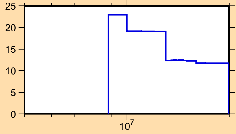
\Delta\sigma/\sigma vs. E for ^{126}\text{La}(n,\text{el.})
