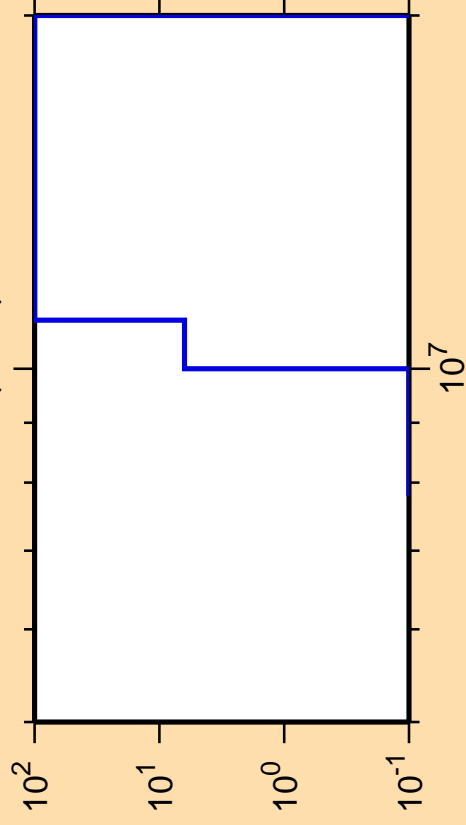
\Delta\sigma/\sigma vs. E for ^{126}\text{La}(n,nd)
