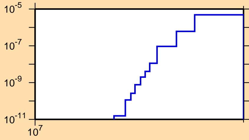
\sigma vs. E for ^{126}\text{La}(n,2n\alpha)
