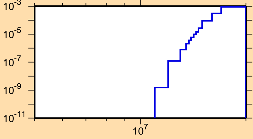
\sigma vs. E for ^{126}\text{La}(n,nd)
