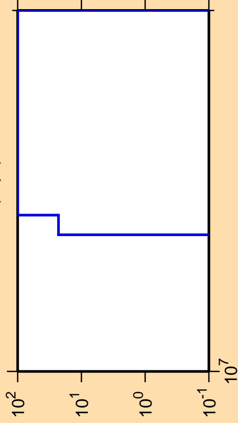
\Delta\sigma/\sigma vs. E for ^{126}\text{La}(n,pt)
