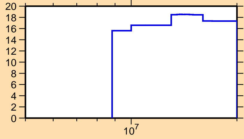
\Delta\sigma/\sigma vs. E for ^{126}\text{La}(n,\text{nonel.})
