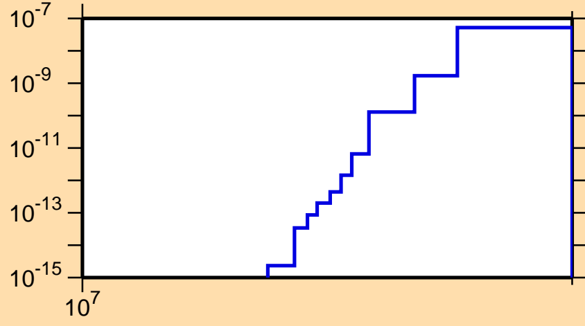
\sigma vs. E for ^{126}\text{La} (mt 34)
