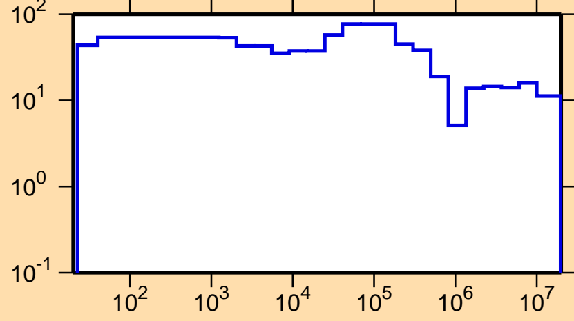
\Delta\sigma/\sigma vs. E for ^{126}\text{La}(n,\text{tot.})
