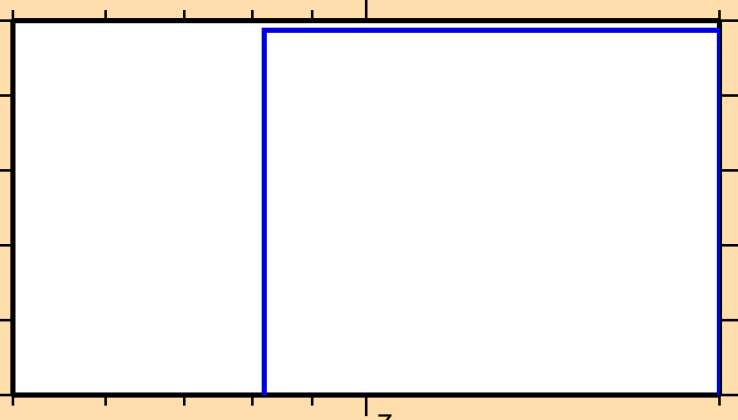
\sigma vs. E for ^{126}\text{La}(\text{mt117})
