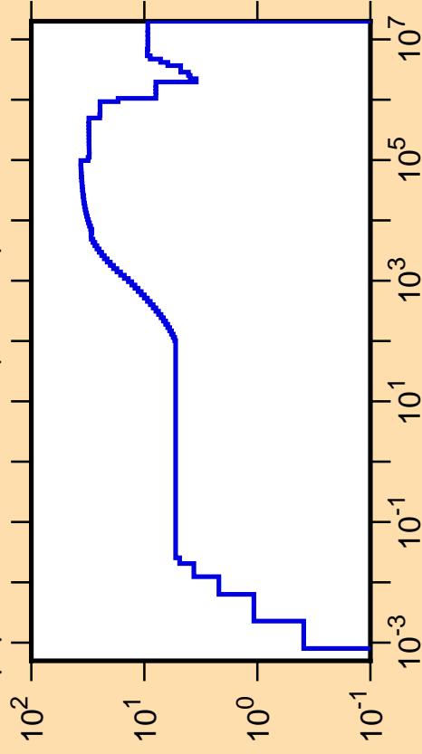
\Delta\mu/\mu vs. E for ^{127}\text{La}(\text{mt251})
