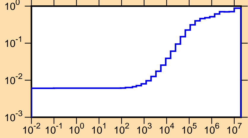
\mu vs. E for ^{127}\text{La}(\text{mt251})
