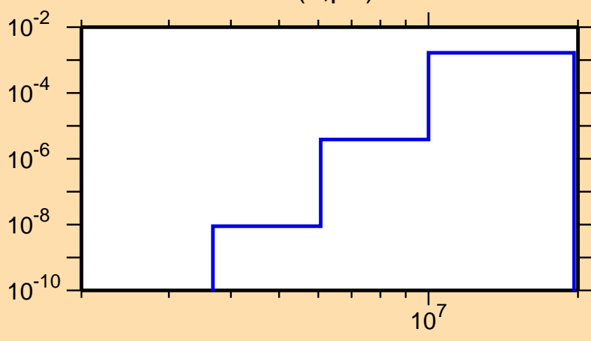
\sigma vs. E for ^{127}\text{La}(n,p\alpha)
