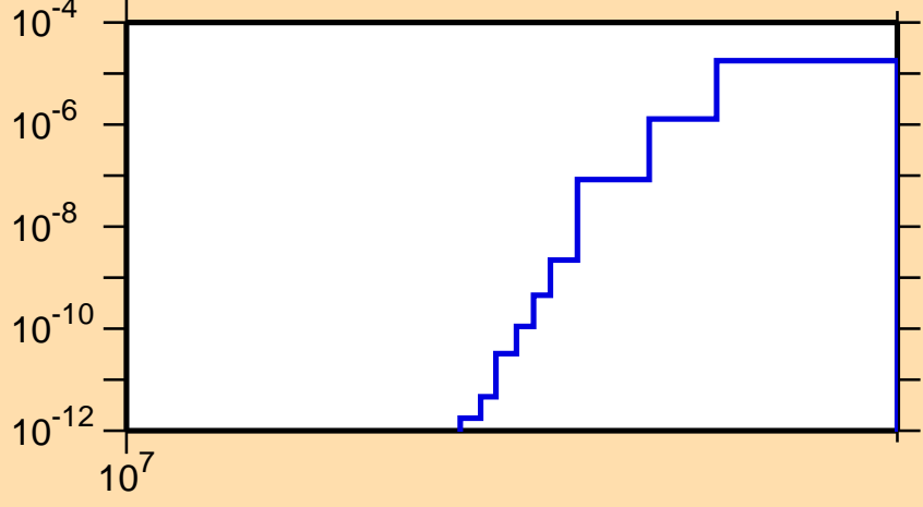
\sigma vs. E for ^{127}\text{La}(n,nd)
