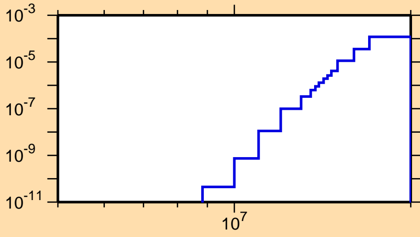
\sigma vs. E for ^{127}\text{La}(n,\text{He}3)
