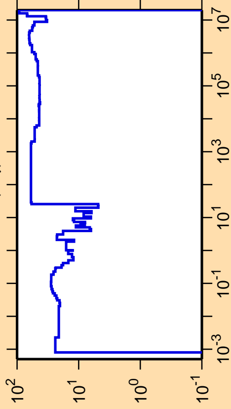
\Delta\sigma/\sigma vs. E for ^{127}\text{La}(n,\gamma)
