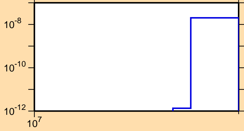
\sigma vs. E for ^{127}\text{La}(n,nt)
