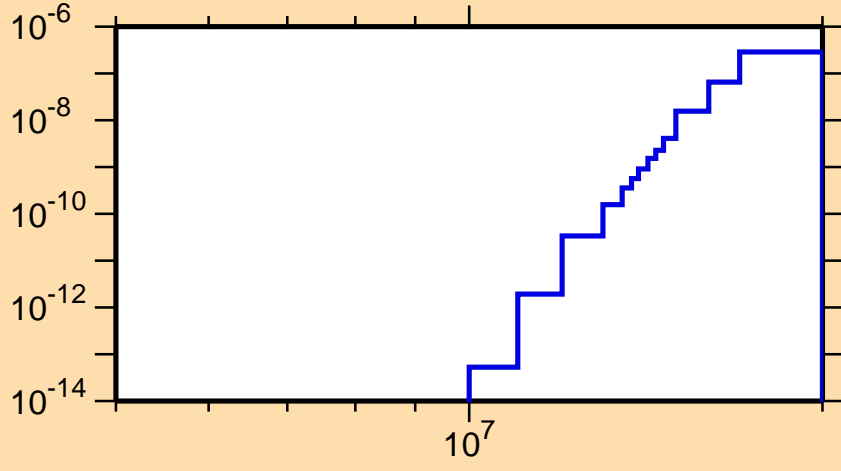
\sigma vs. E for ^{127}\text{La}(\text{mt117})
