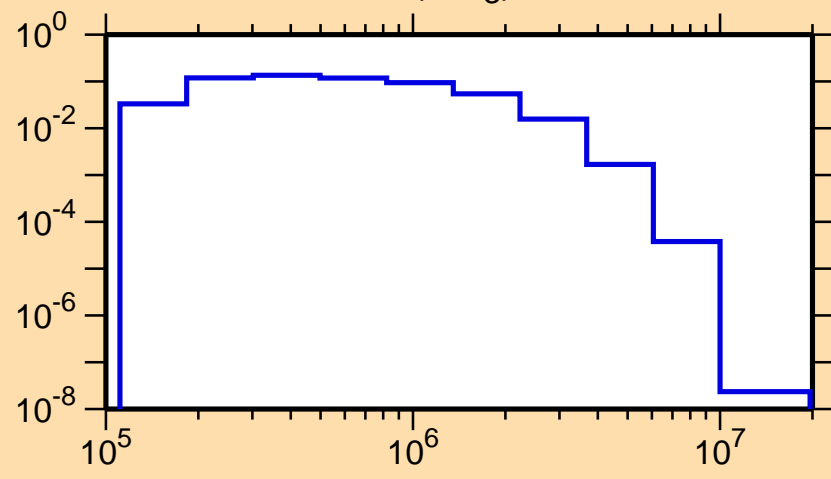
\sigma vs. E for ^{127}\text{La}(n,n_3)
