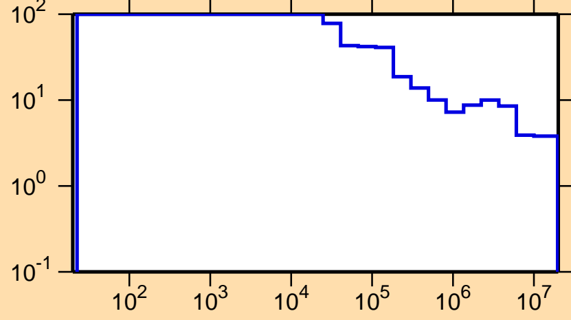
\Delta\sigma/\sigma vs. E for ^{127}\text{La}(n,\text{tot.})
