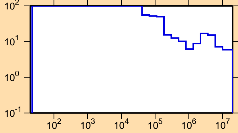
\Delta\sigma/\sigma vs. E for ^{127}\text{La}(n,\text{el.})
