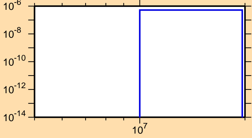
\sigma vs. E for ^{127}\text{La}(n,pd)
