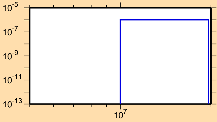
\sigma vs. E for ^{127}\text{La}(\text{mt } 45)
