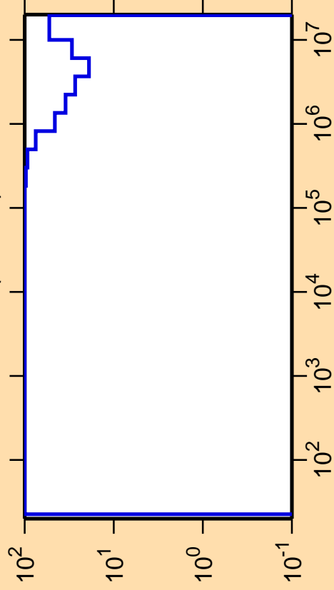
\Delta\sigma/\sigma vs. E for ^{127}\text{La}(n,\text{inel.})
