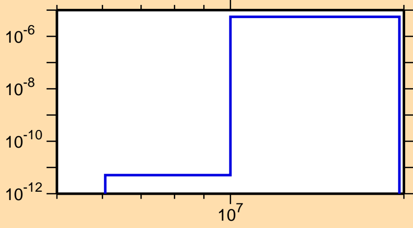
\sigma vs. E for ^{127}\text{La}(n,\text{He}3)
