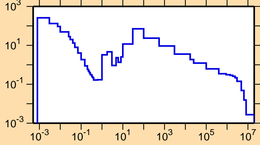
\sigma vs. E for ^{127}\text{La}(n,\gamma)
