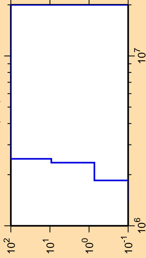
\Delta\sigma/\sigma vs. E for ^{127}\text{La}(n,d)
