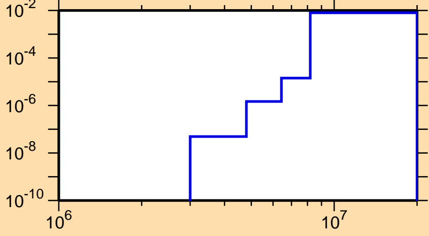
\sigma vs. E for ^{127}\text{La}(n,d)
