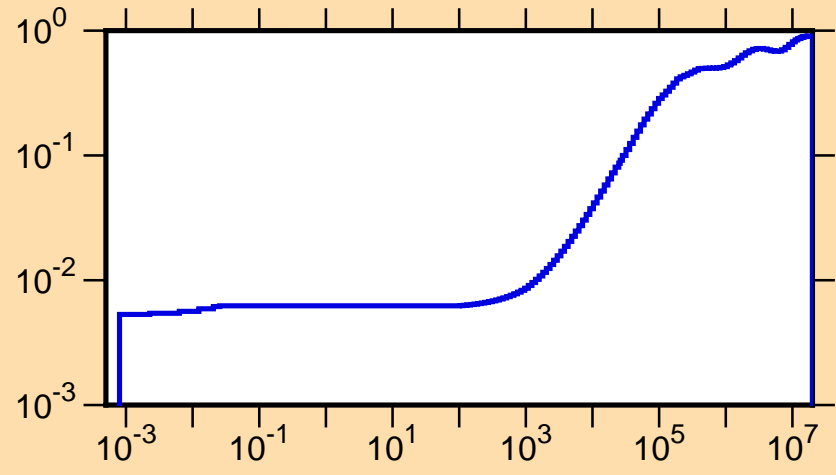
\mu vs. E for ^{128}\text{La}(\text{mt251})
