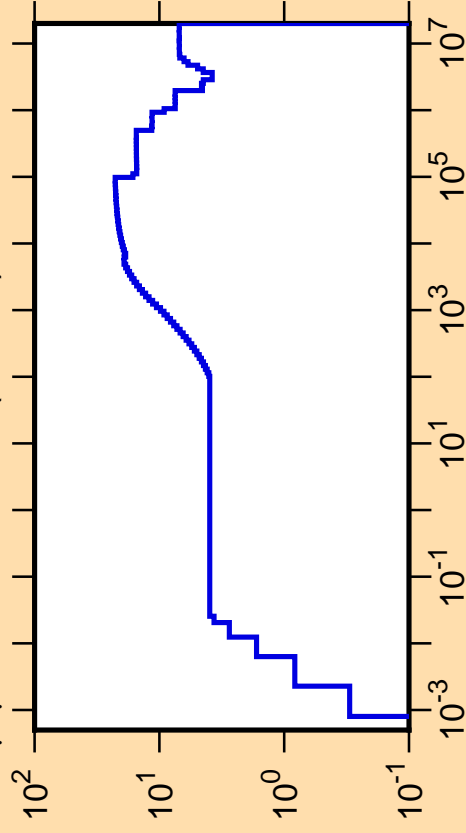
\Delta\mu/\mu vs. E for ^{128}\text{La}(\text{mt251})
