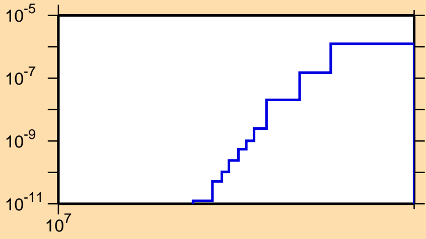
\sigma vs. E for ^{128}\text{La}(n,pd)
