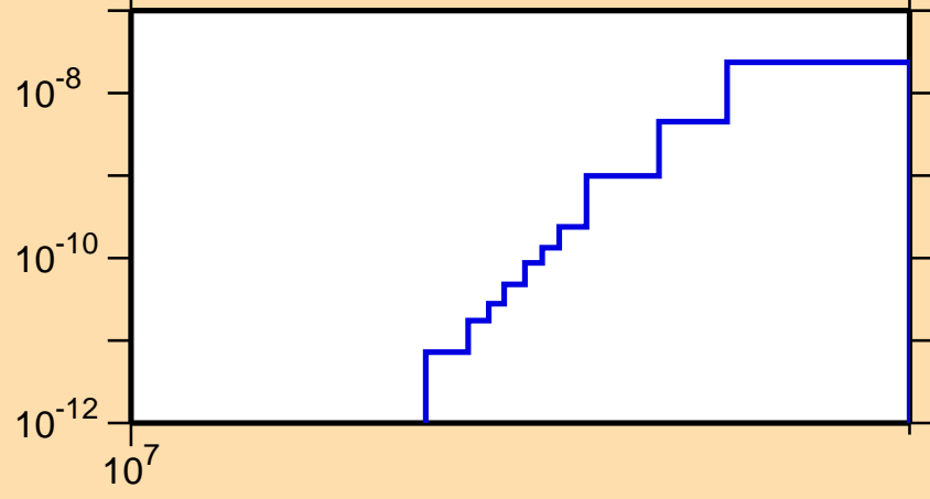
\sigma vs. E for ^{128}\text{La}(\text{mt117})
