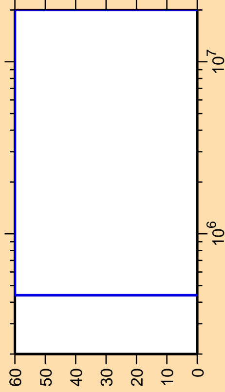
\Delta\sigma/\sigma vs. E for ^{128}\text{La}(n,\alpha)
