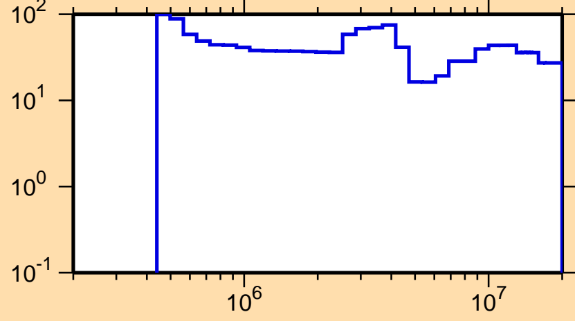
\Delta\sigma/\sigma vs. E for ^{128}\text{La}(n,n\text{cont.})
