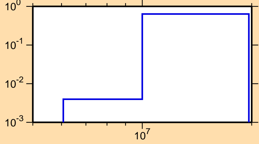
\sigma vs. E for ^{128}\text{La}(n,2n)
