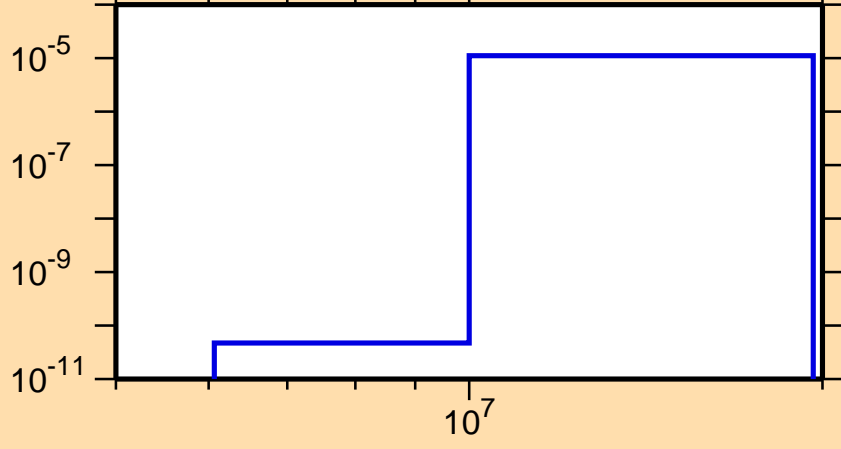
\sigma vs. E for ^{128}\text{La}(n,\text{He}3)
