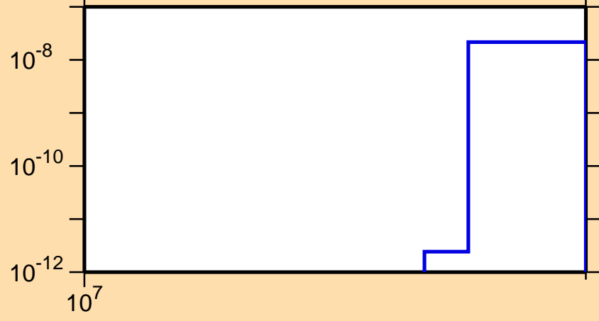
\sigma vs. E for ^{128}\text{La}(n,nt)
