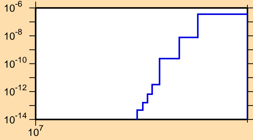
\sigma vs. E for ^{128}\text{La}(n,pt)
