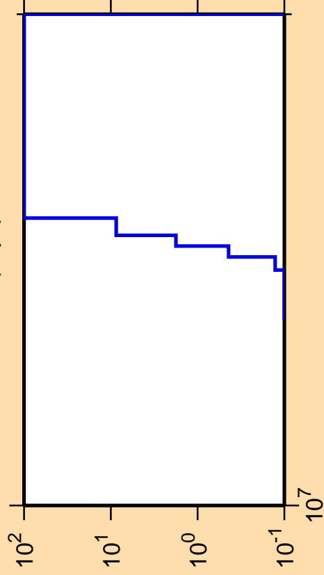
\Delta\sigma/\sigma vs. E for ^{128}\text{La}(n,pt)
