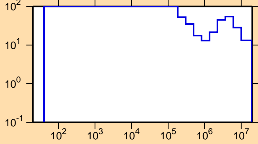
\Delta\sigma/\sigma vs. E for ^{128}\text{La}(n,\text{el.})
