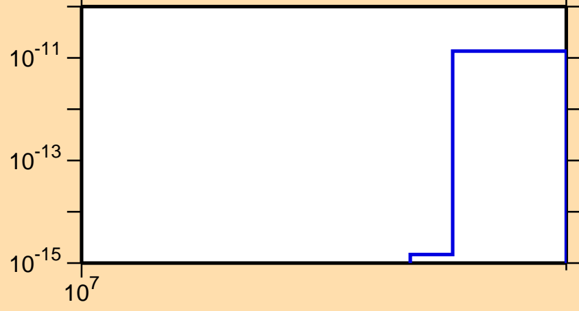
\sigma vs. E for ^{129}\text{La}(n,\text{pt})
