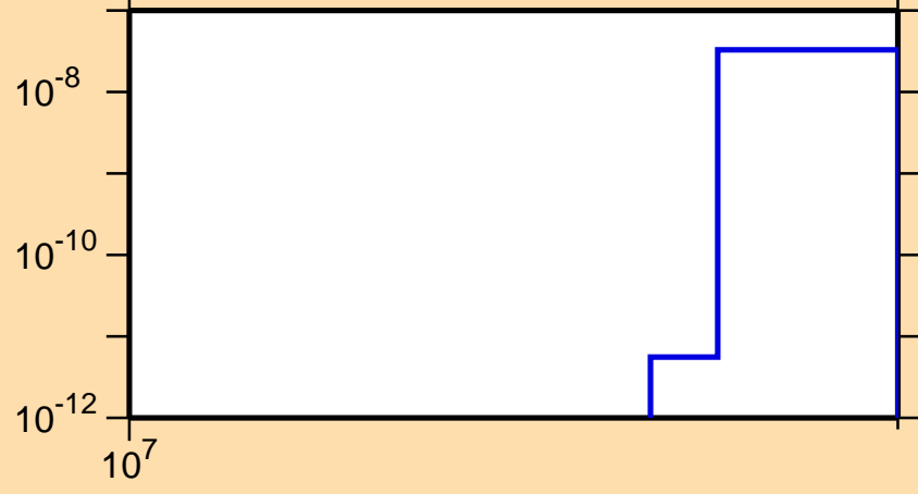
\sigma vs. E for ^{129}\text{La}(n,nt)
