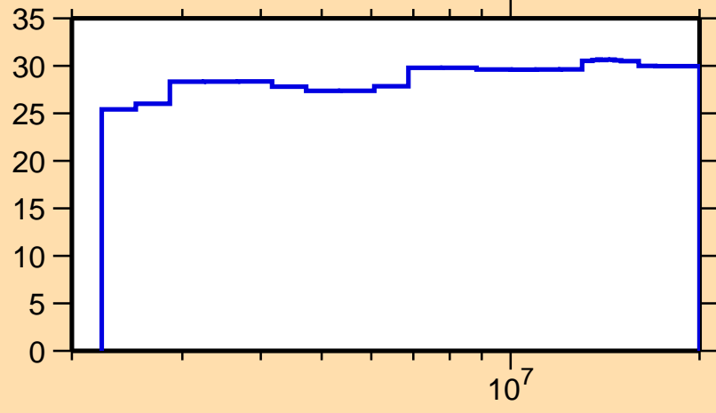
\Delta\sigma/\sigma vs. E for ^{129}\text{La}(n,n_1)
