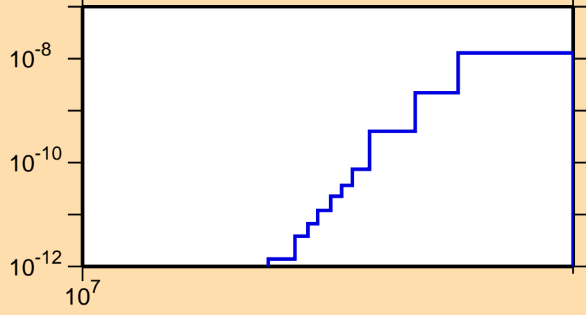
\sigma vs. E for ^{129}\text{La}(\text{mt117})
