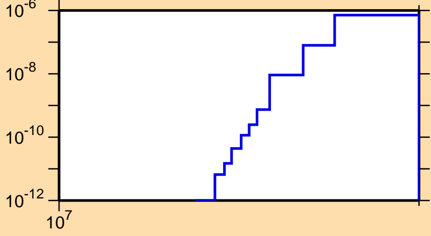
\sigma vs. E for ^{129}\text{La}(n,pd)
