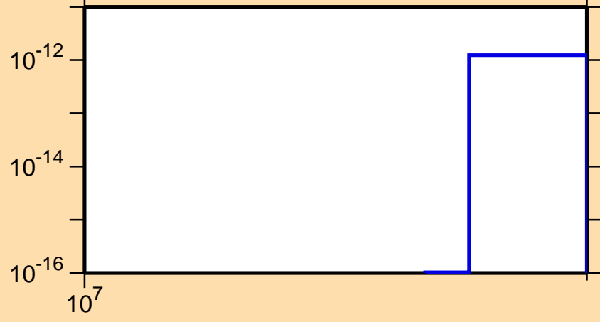
\sigma vs. E for ^{129}\text{La} (mt 34)
