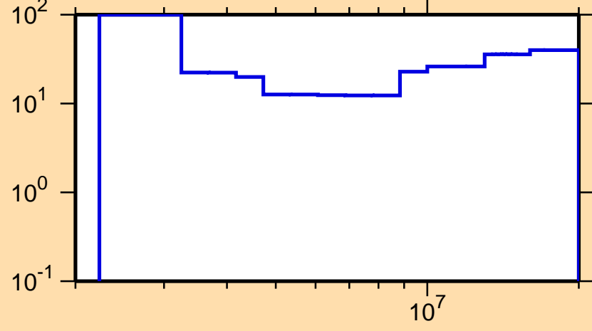
\Delta\sigma/\sigma vs. E for ^{129}\text{La}(n,n\text{cont.})
