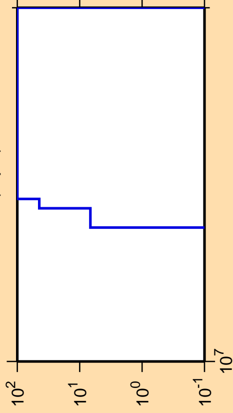
\Delta\sigma/\sigma vs. E for ^{129}\text{La}(n,pd)
