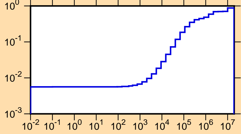
\mu vs. E for ^{129}\text{La}(\text{mt251})
