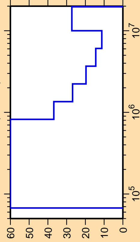
\Delta\sigma/\sigma vs. E for ^{129}\text{La}(n,\text{inel.})
