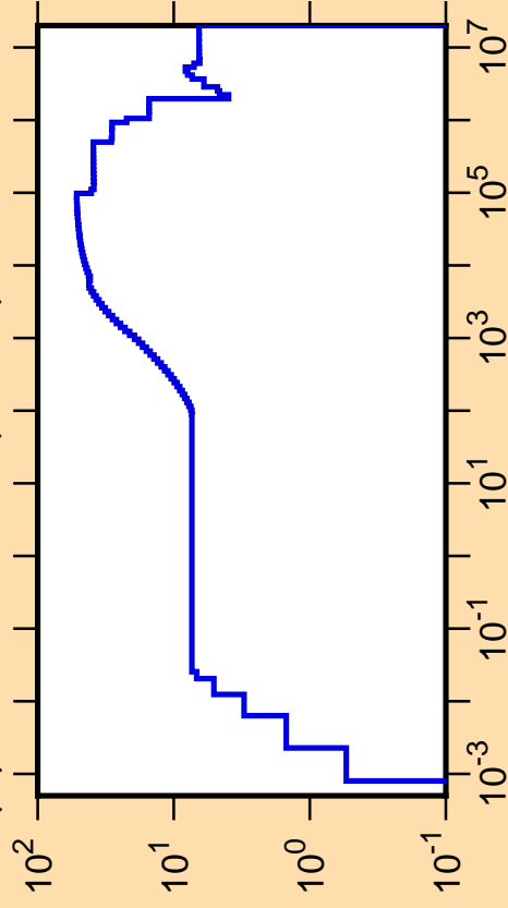
\Delta\mu/\mu vs. E for ^{130}\text{La}(\text{mt251})
