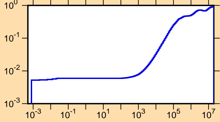
\mu vs. E for ^{130}\text{La}(\text{mt251})
