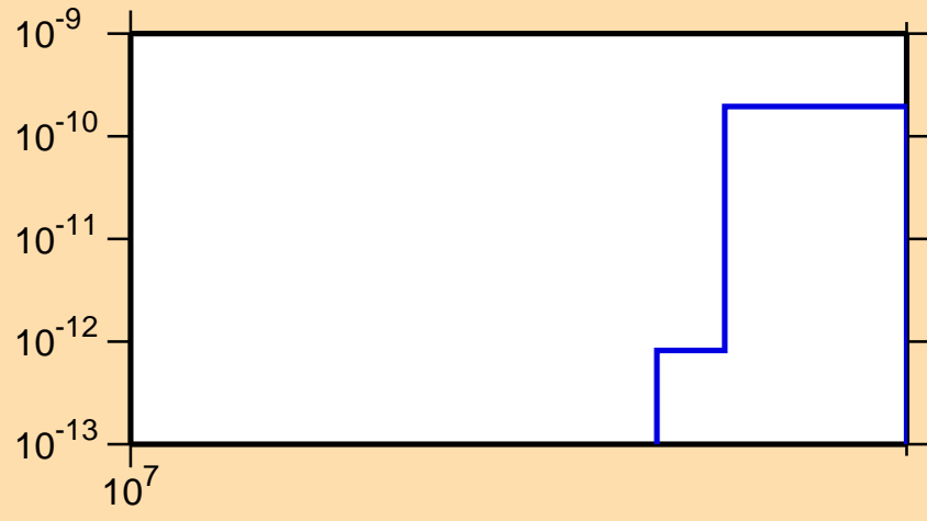
\sigma vs. E for ^{130}\text{La} (mt 34)
