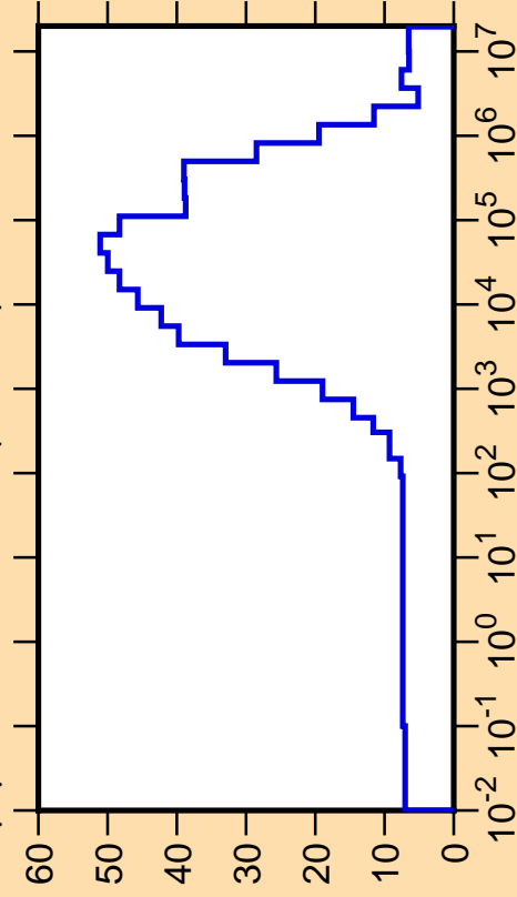
\Delta\mu/\mu vs. E for ^{130}\text{La}(\text{mt251})
