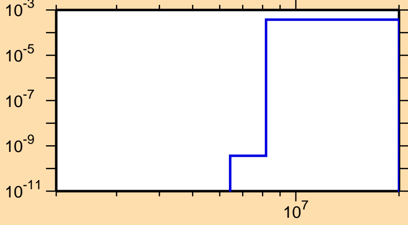
\sigma vs. E for ^{130}\text{La}(n,t)
