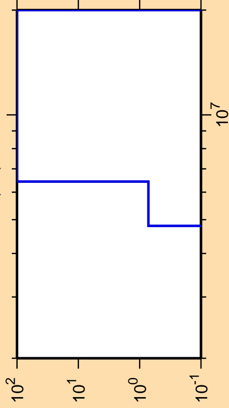
\Delta\sigma/\sigma vs. E for ^{130}\text{La}(n,t)
