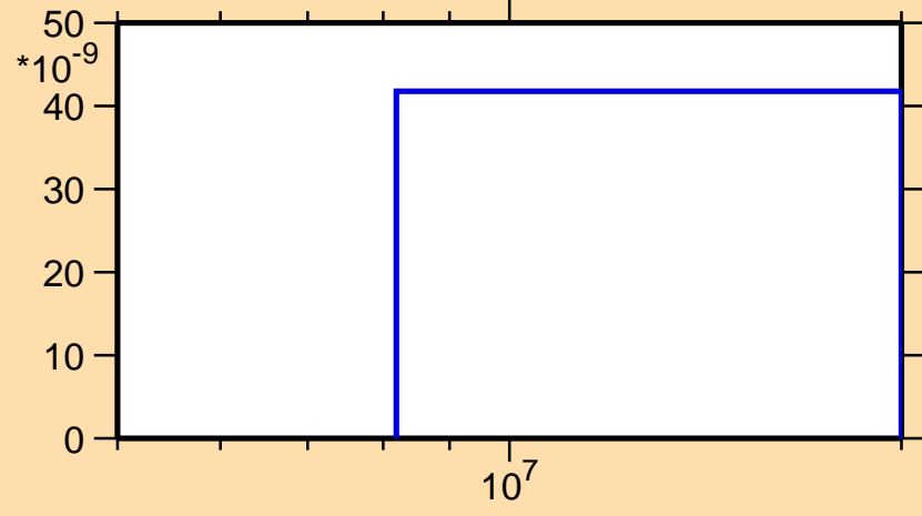
\sigma vs. E for ^{130}\text{La}(n,2n\alpha)
