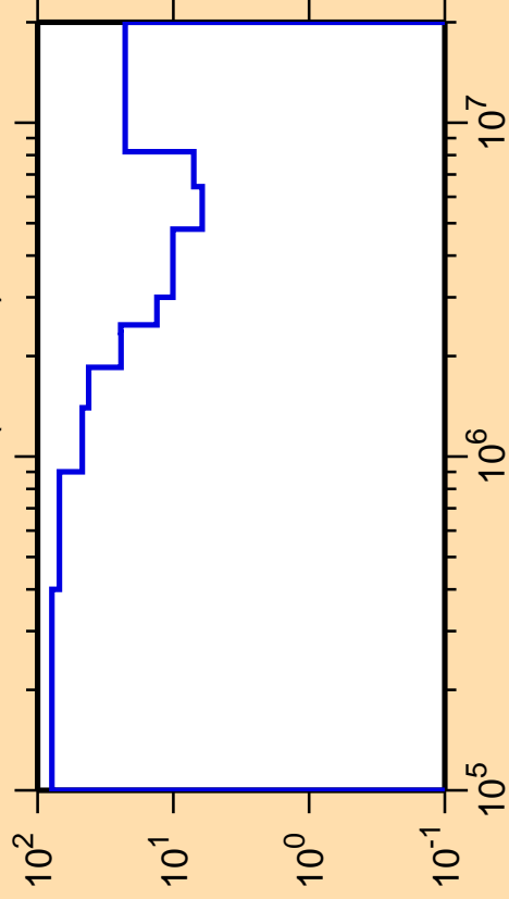
\Delta\sigma/\sigma vs. E for ^{130}\text{La}(n,\text{inel.})
