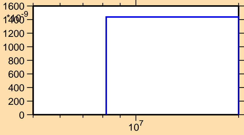
\sigma vs. E for ^{130}\text{La}(n,\text{He}3)
