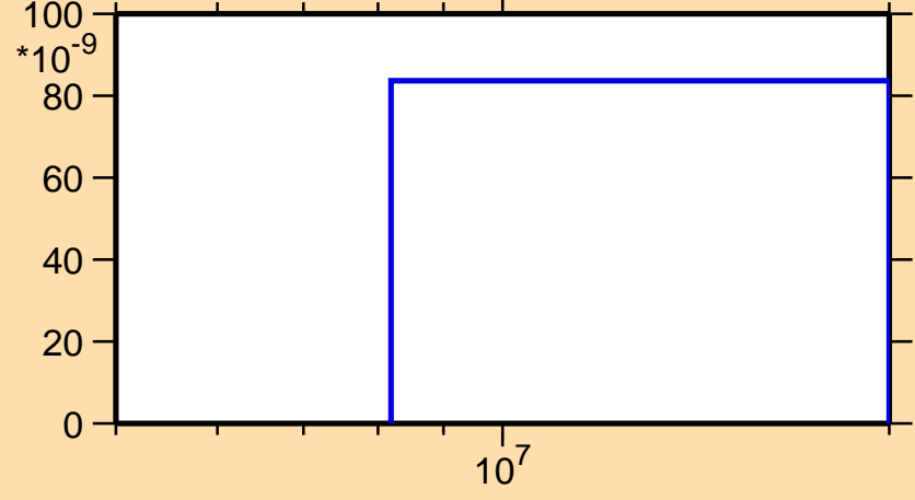
\sigma vs. E for ^{130}\text{La}(n,3n)
