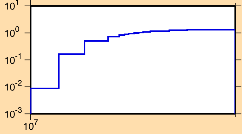
\sigma vs. E for ^{131}\text{La}(n,2n)
