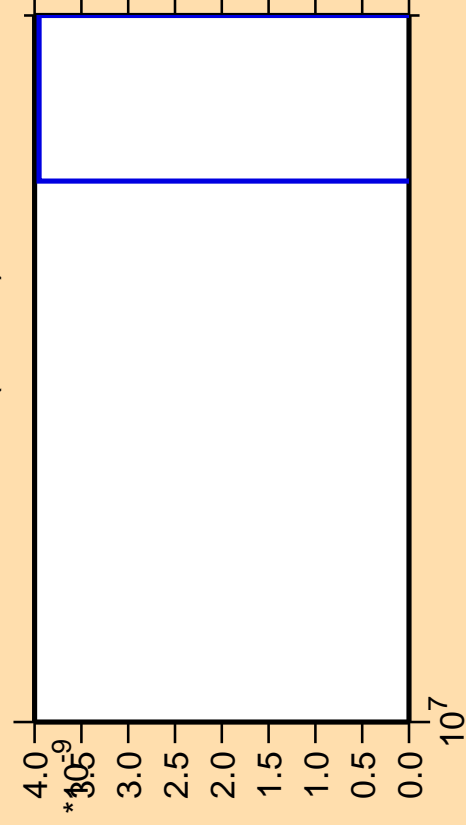
\Delta\sigma/\sigma vs. E for ^{131}\text{La} (mt 11)
