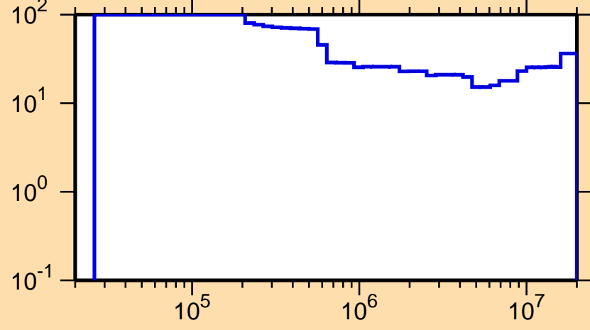
\Delta\sigma/\sigma vs. E for ^{131}\text{La}(n,\text{inel.})
