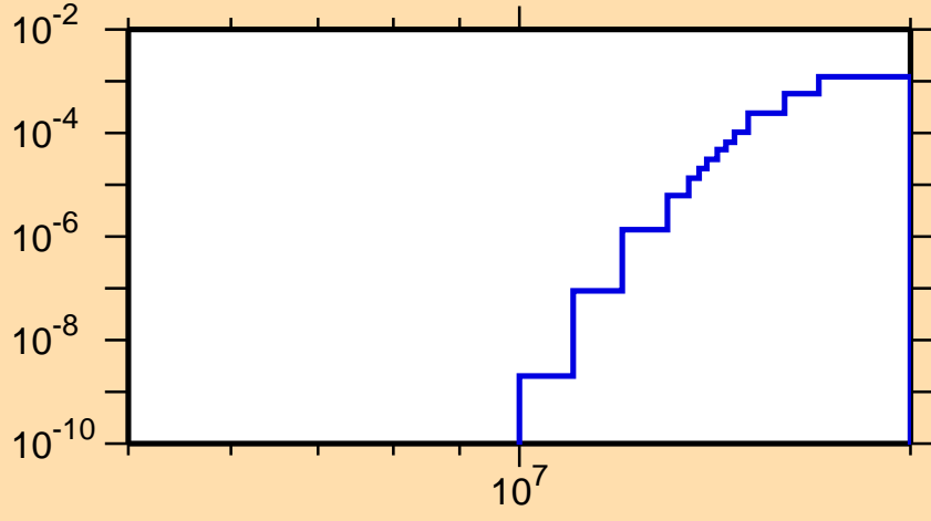
\sigma vs. E for ^{131}\text{La}(n,t)
