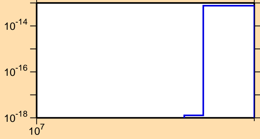
\sigma vs. E for ^{131}\text{La} (mt 34)
