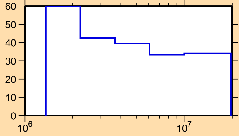
\Delta\sigma/\sigma vs. E for ^{131}\text{La}(n,ncont.)
