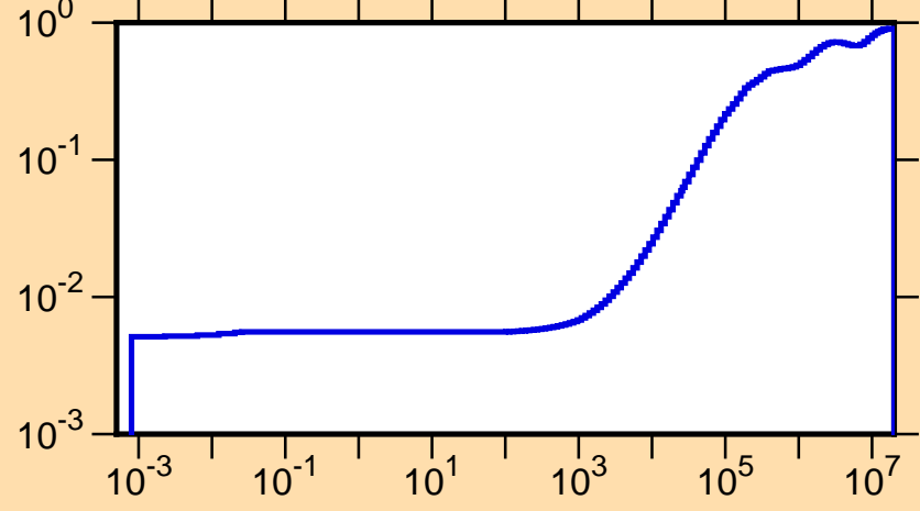
\mu vs. E for ^{132}\text{La}(\text{mt251})
