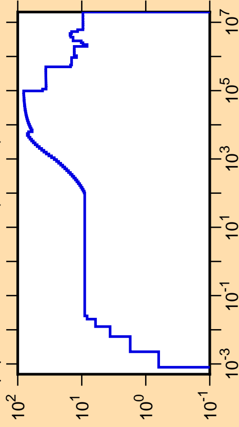
\Delta\mu/\mu vs. E for ^{132}\text{La}(\text{mt251})
