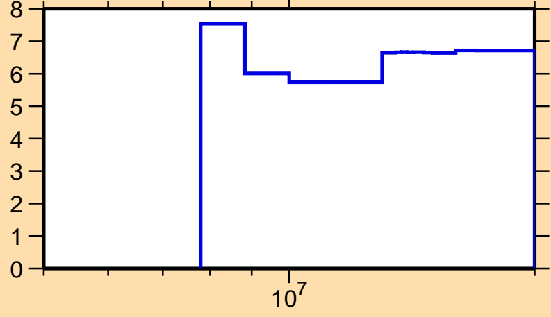
\Delta\sigma/\sigma vs. E for ^{132}\text{La}(n,\text{nonel.})
