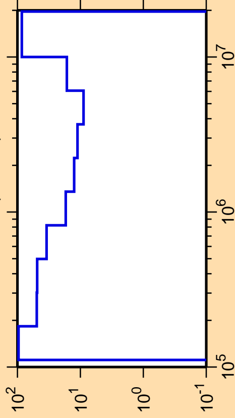
\Delta\sigma/\sigma vs. E for ^{132}\text{La}(n,\text{inel.})
