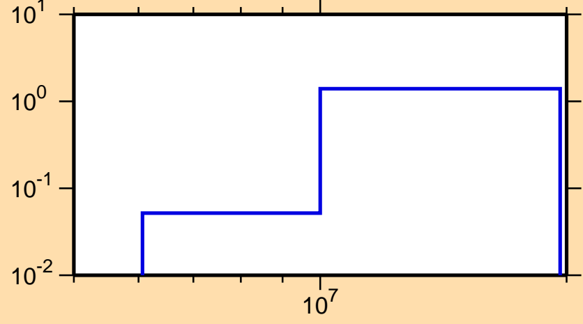
\sigma vs. E for ^{132}\text{La}(n,2n)
