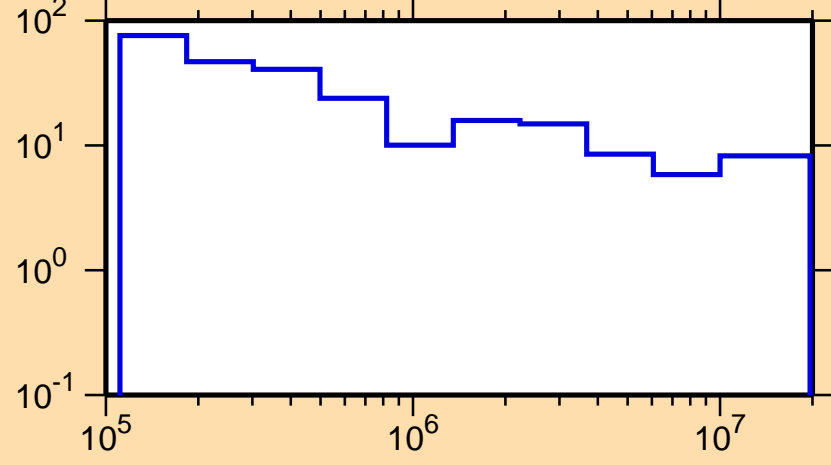
\Delta\sigma/\sigma vs. E for ^{132}\text{La}(n,\text{tot.})
