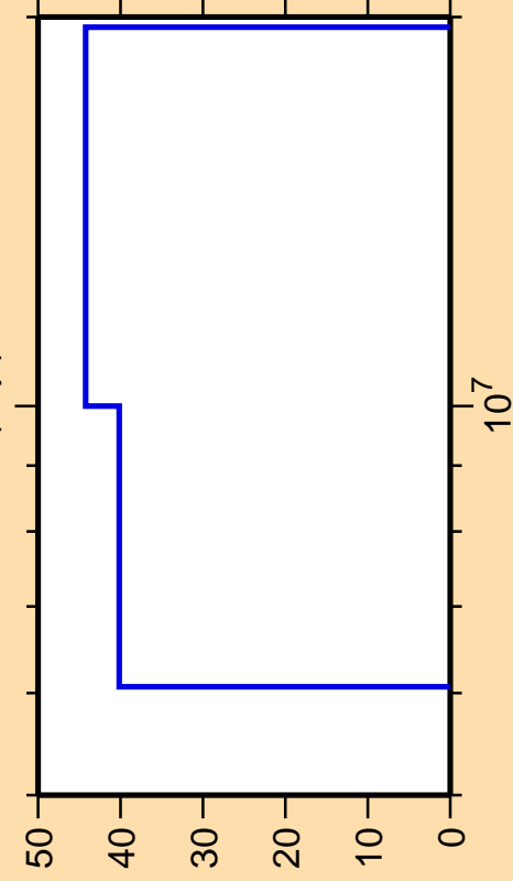
\Delta\sigma/\sigma vs. E for ^{132}\text{La}(n,p)
