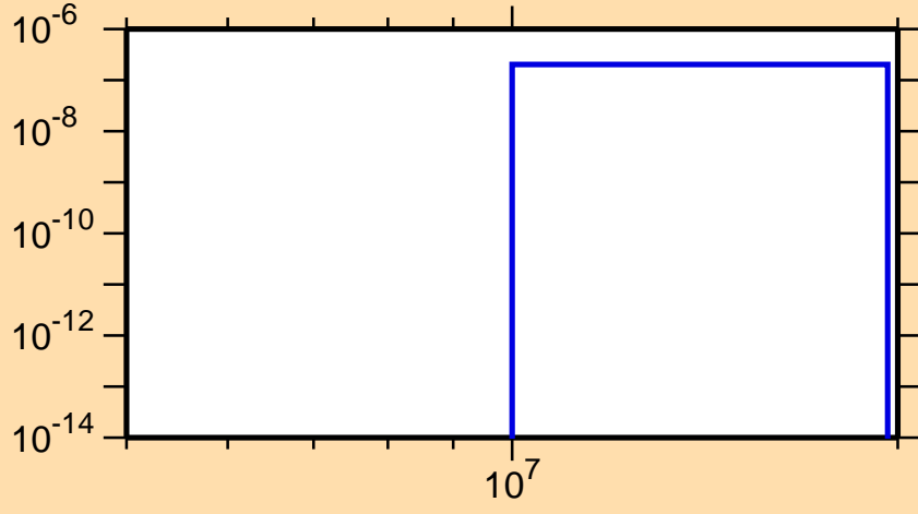
\sigma vs. E for ^{132}\text{La}(n,\text{He3})
