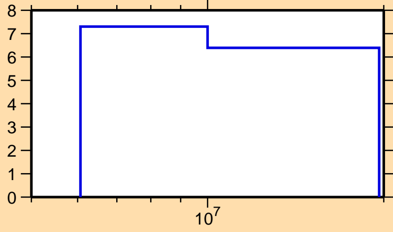
\Delta\sigma/\sigma vs. E for ^{132}\text{La}(n,\text{nonel.})
