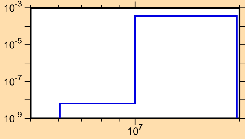
\sigma vs. E for ^{132}\text{La}(n,t)
