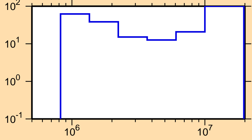
\Delta\sigma/\sigma vs. E for ^{132}\text{La}(n,n\text{cont.})
