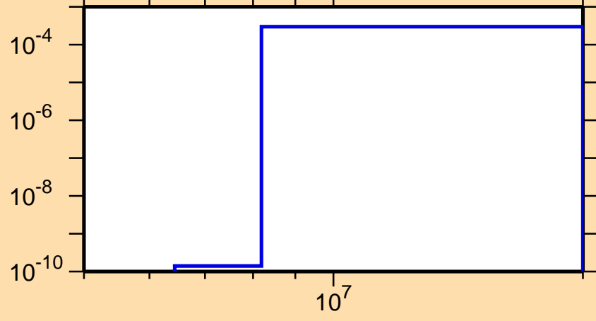
\sigma vs. E for ^{132}\text{La}(n,t)
