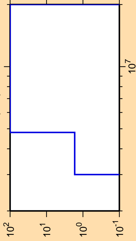
\Delta\sigma/\sigma vs. E for ^{132}\text{La}(n,d)
