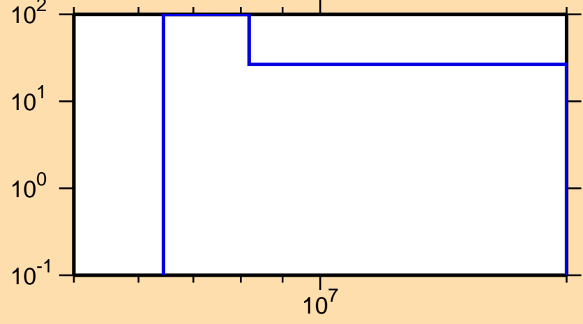
\Delta\sigma/\sigma vs. E for ^{132}\text{La}(n,2n)
