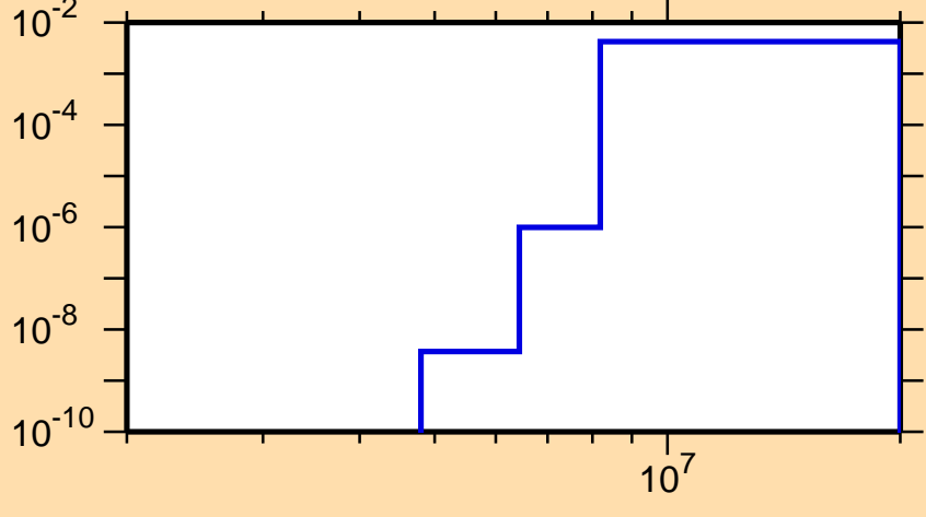
\sigma vs. E for ^{132}\text{La}(n,d)
