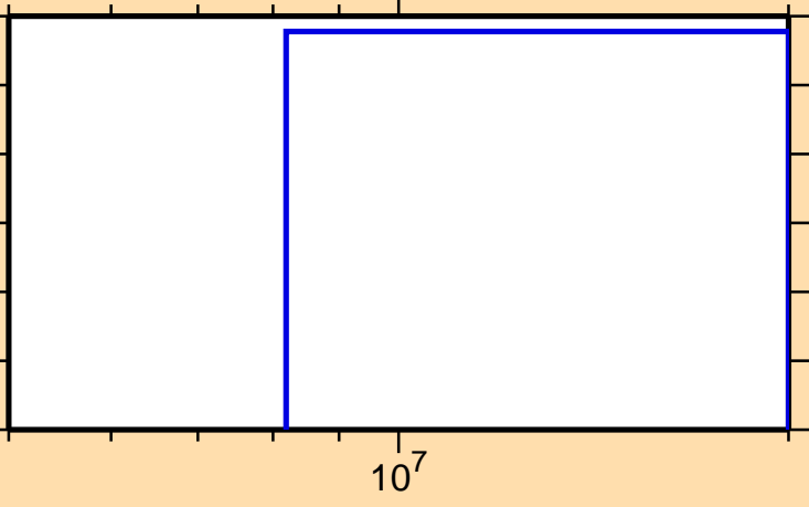
\sigma vs. E for ^{132}\text{La}(n,\text{He3})
