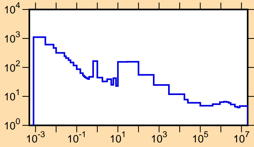
\sigma vs. E for ^{132}\text{La}(n,\text{tot.})
