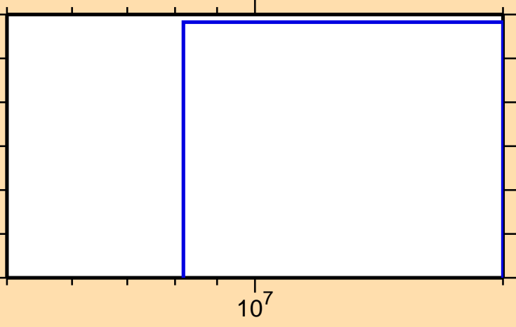
\sigma vs. E for ^{132}\text{La}(\text{mt117})
