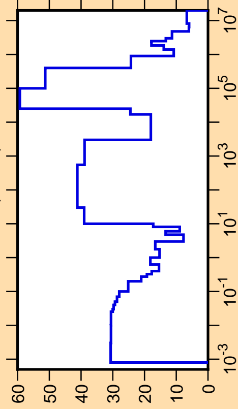
\Delta\sigma/\sigma vs. E for ^{132}\text{La}(n,\text{tot.})
