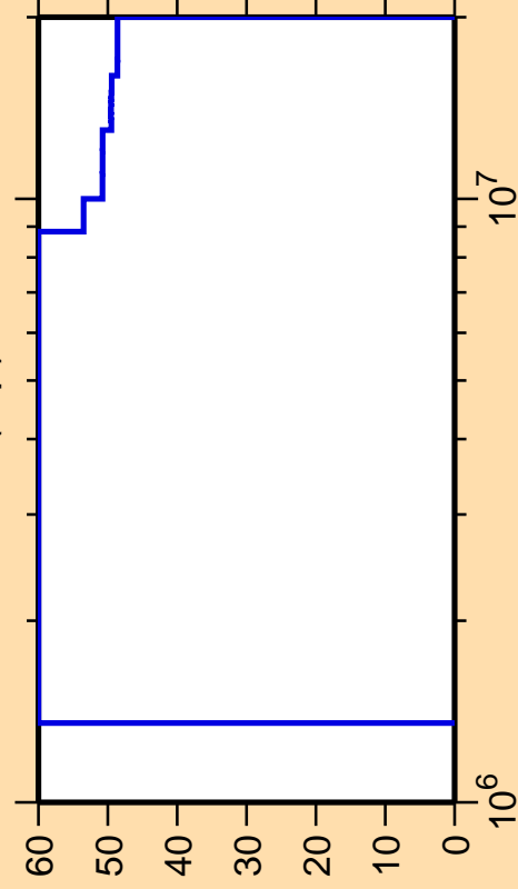
\Delta\sigma/\sigma vs. E for ^{133}\text{La}(n,p)
