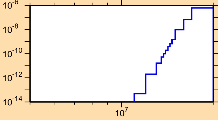
\sigma vs. E for ^{133}\text{La}(n,\text{He3})
