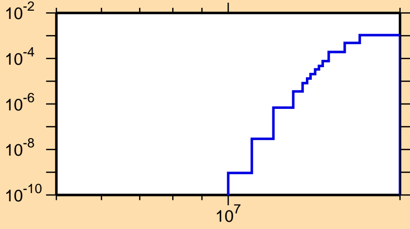
\sigma vs. E for ^{133}\text{La}(n,t)
