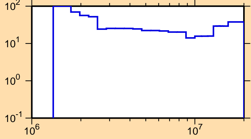
\Delta\sigma/\sigma vs. E for ^{133}\text{La}(n,ncont.)
