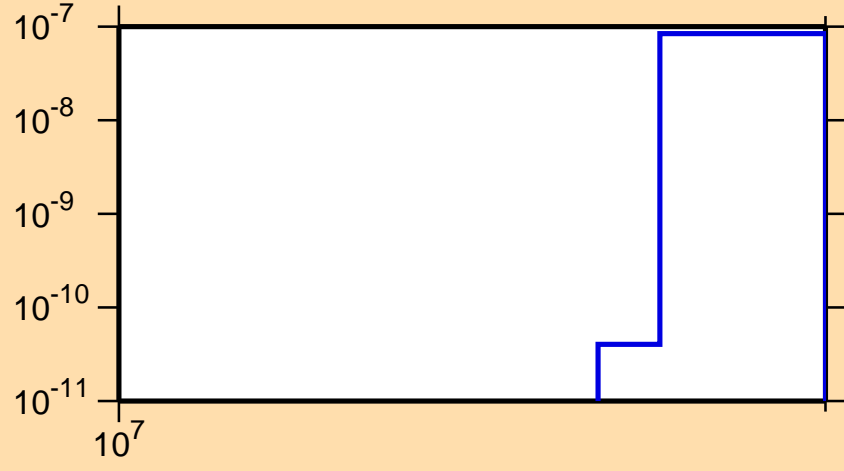
\sigma vs. E for ^{133}\text{La}(n,nt)
