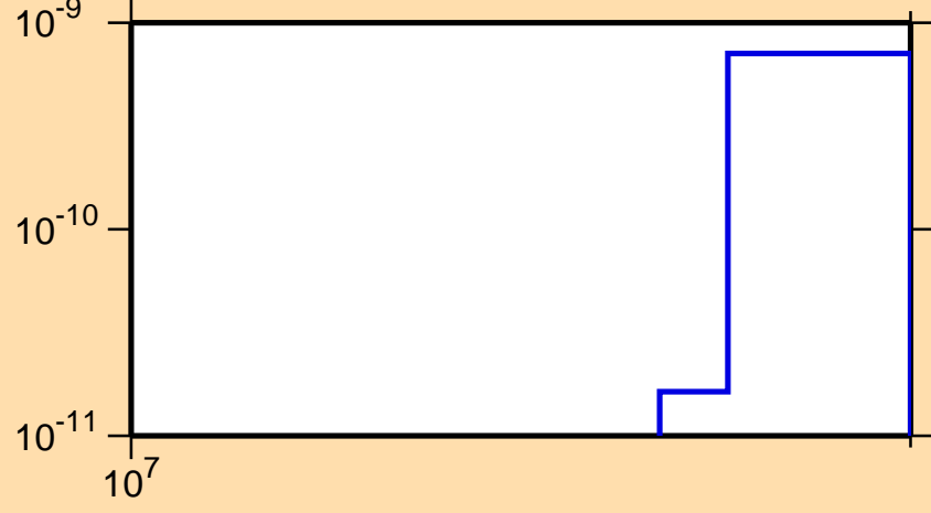
\sigma vs. E for ^{133}\text{La} (mt 45)
