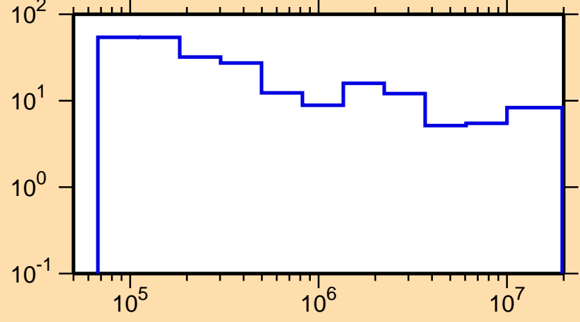
\Delta\sigma/\sigma vs. E for ^{133}\text{La}(n,\text{tot.})
