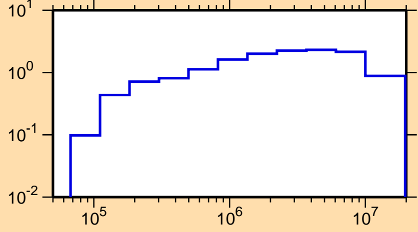
\sigma vs. E for ^{133}\text{La}(n,\text{inel.})
