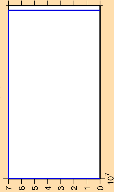
\Delta\sigma/\sigma vs. E for ^{133}\text{La}(n,pd)
