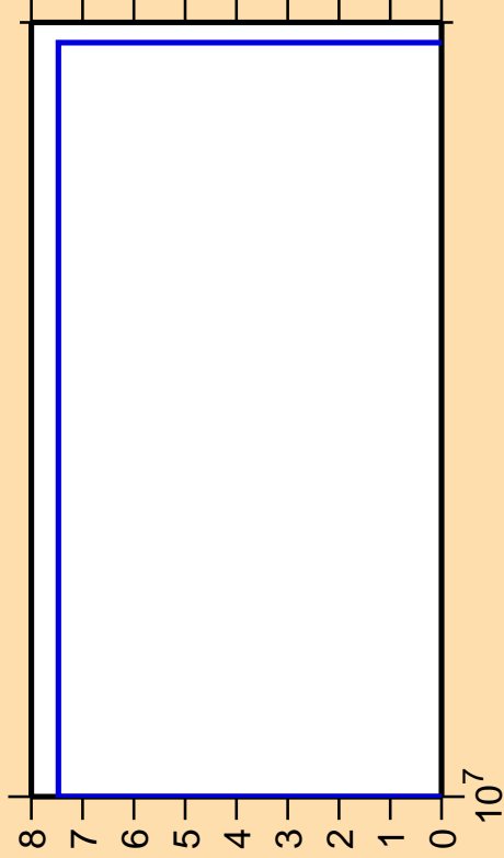
\Delta\sigma/\sigma vs. E for ^{133}\text{La} (mt 45)
