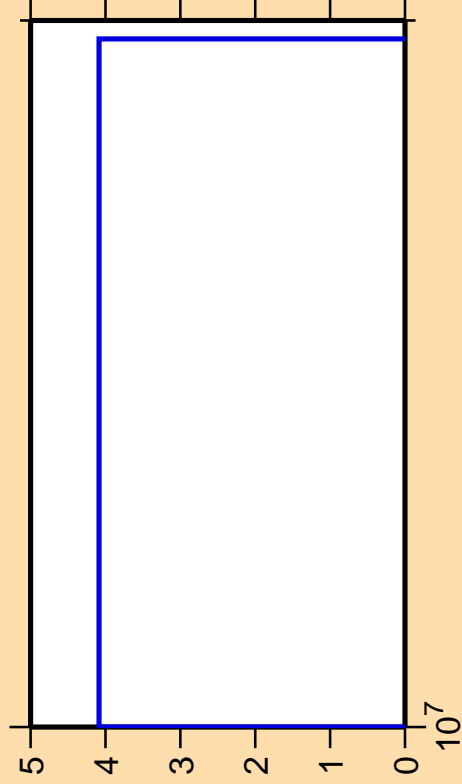
\Delta\sigma/\sigma vs. E for ^{133}\text{La}(\text{mt117})
