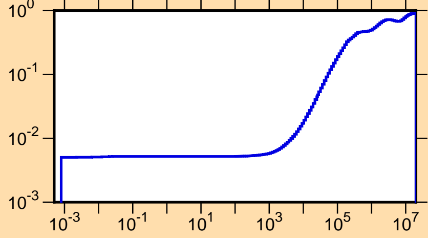
\mu vs. E for ^{134}\text{La}(\text{mt251})
