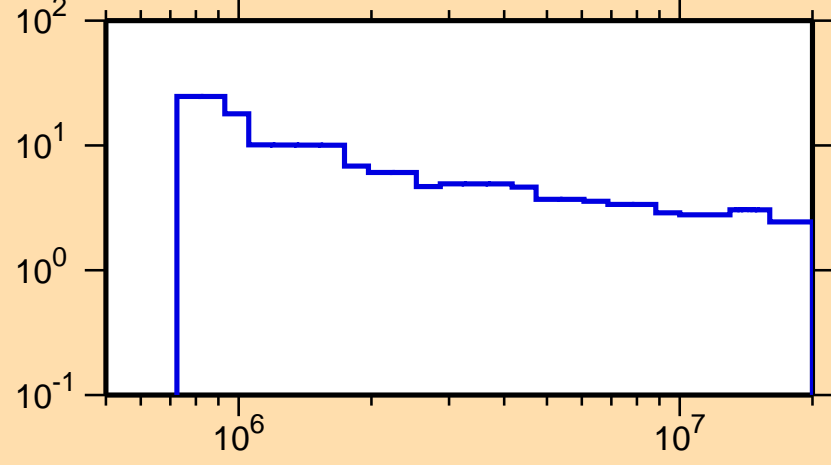
\Delta\sigma/\sigma vs. E for ^{134}\text{La}(n,\text{nonel.})
