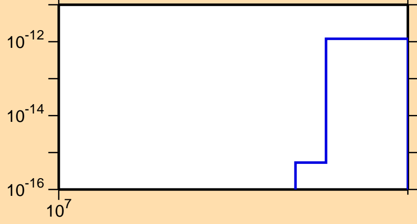
\sigma vs. E for ^{134}\text{La} (mt 34)
