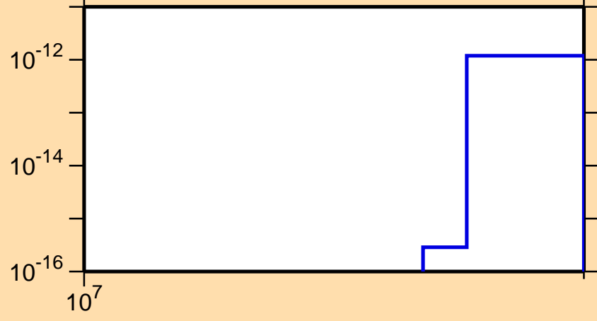
\sigma vs. E for ^{134}\text{La}(n,\text{pt})
