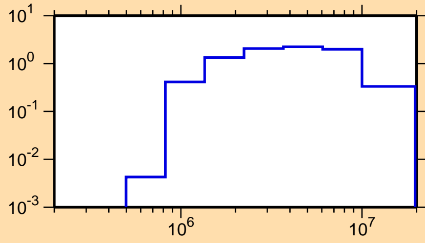
\sigma vs. E for ^{134}\text{La}(n,n\text{cont.})
