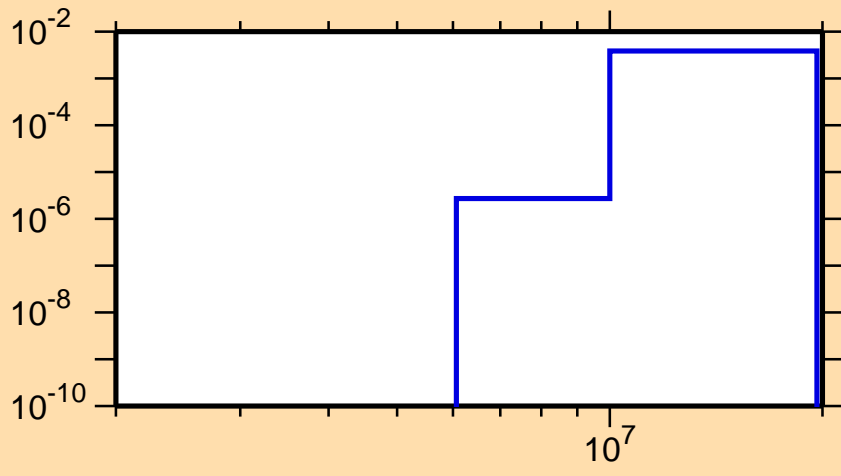
\sigma vs. E for ^{134}\text{La}(n,d)
