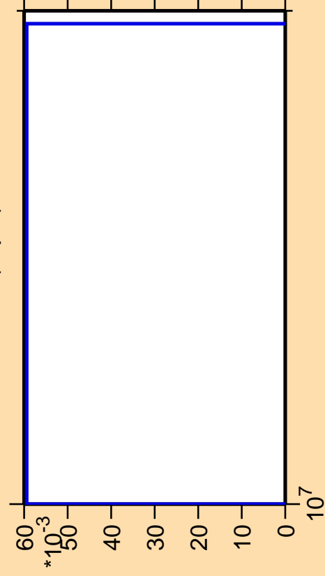
\Delta\sigma/\sigma vs. E for ^{134}\text{La}(n,\text{pd})
