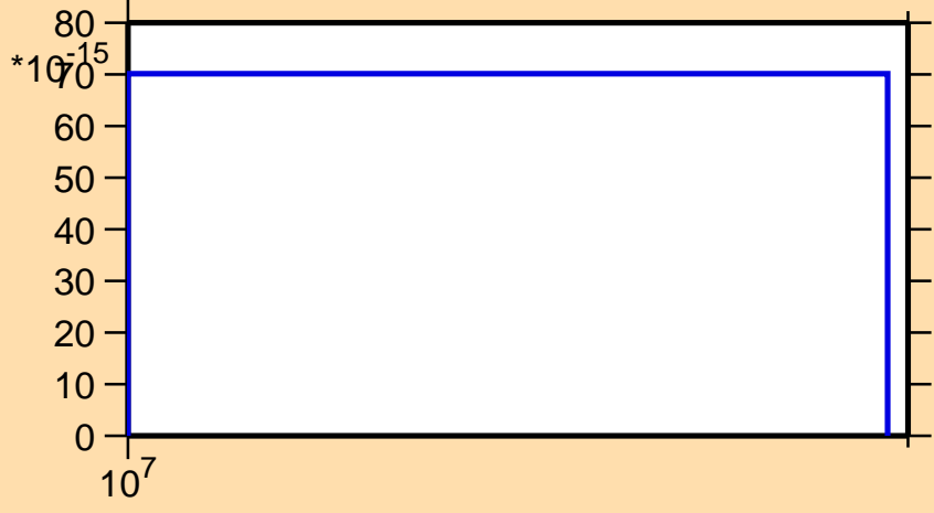
\sigma vs. E for ^{134}\text{La}(n,\text{pd})
