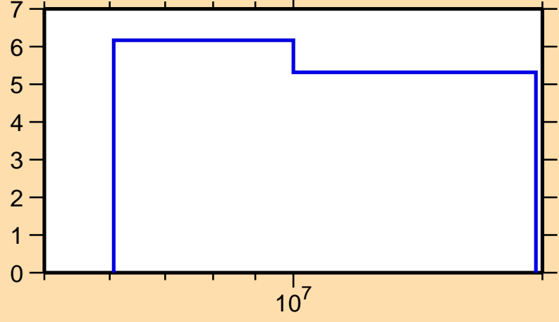
\Delta\sigma/\sigma vs. E for ^{134}\text{La}(n,2n)
