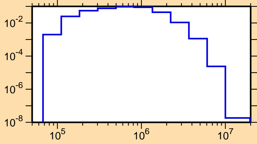
\sigma vs. E for ^{134}\text{La}(n,n_3)
