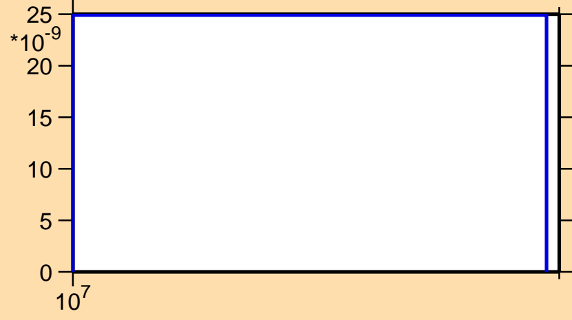
\sigma vs. E for ^{134}\text{La}(n,2n\alpha)
