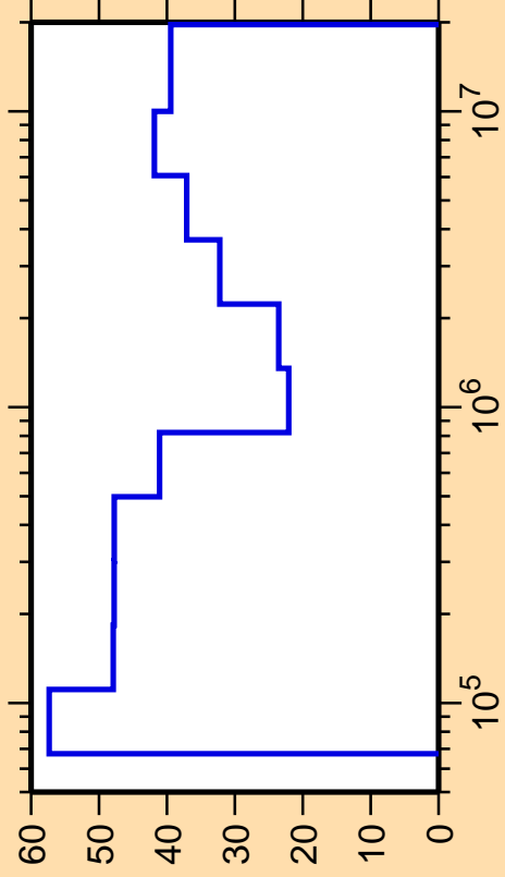
\Delta\sigma/\sigma vs. E for ^{134}\text{La}(n,n_3)
