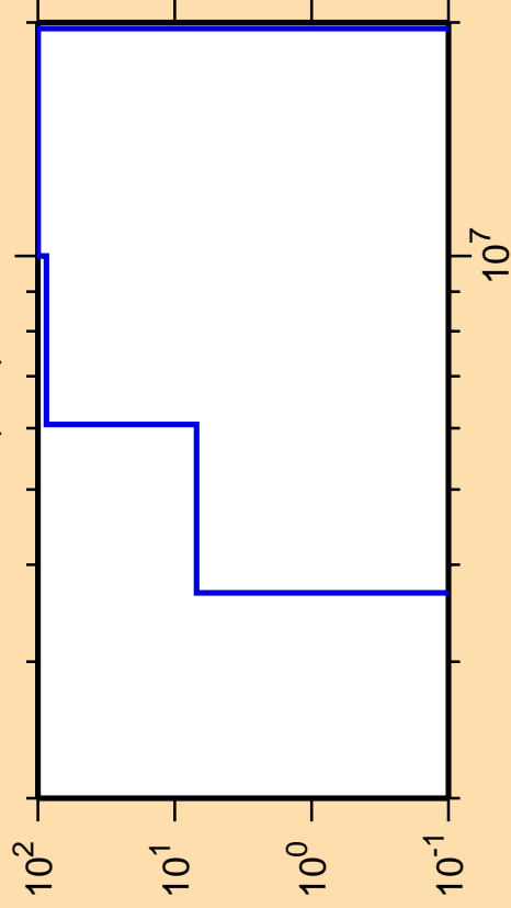
\Delta\sigma/\sigma vs. E for ^{134}\text{La}(n,d)
