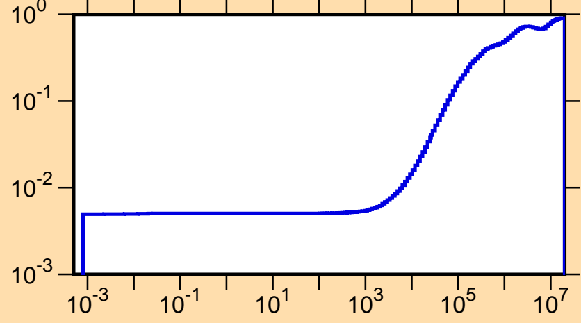
\mu vs. E for ^{136}\text{La}(\text{mt251})
