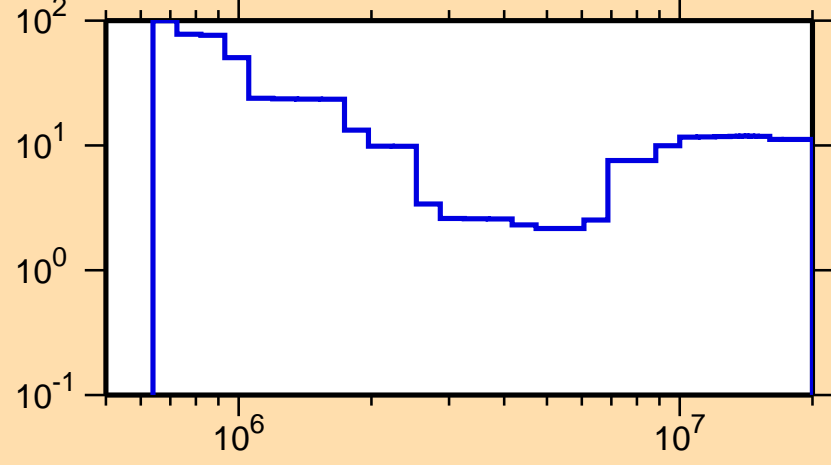
\Delta\sigma/\sigma vs. E for ^{136}\text{La}(n,n\text{cont.})
