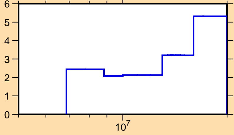
\Delta\sigma/\sigma vs. E for ^{136}\text{La}(n,\text{el.})
