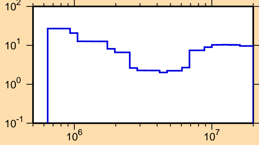
\Delta\sigma/\sigma vs. E for ^{136}\text{La}(n,\text{inel.})
