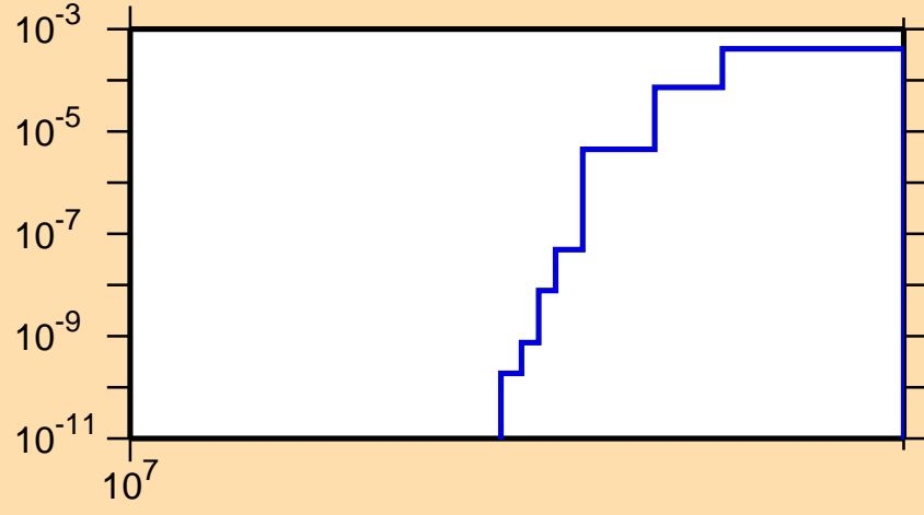
\sigma vs. E for ^{136}\text{La}(n,2np)
