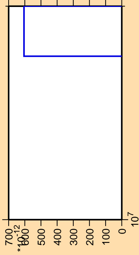
\Delta\sigma/\sigma vs. E for ^{136}\text{La} (mt 11)
