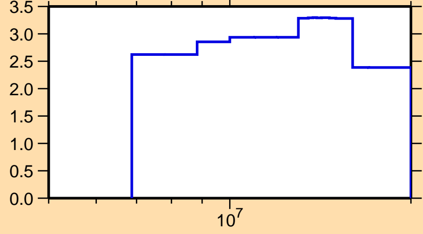
\Delta\sigma/\sigma vs. E for ^{136}\text{La}(n,\text{nonel.})
