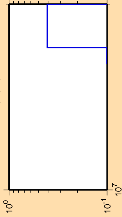
\Delta\sigma/\sigma vs. E for ^{136}\text{La}(n,pd)
