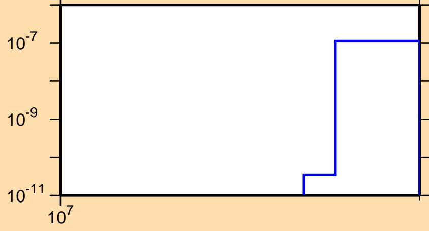
\sigma vs. E for ^{136}\text{La}(n,nt)
