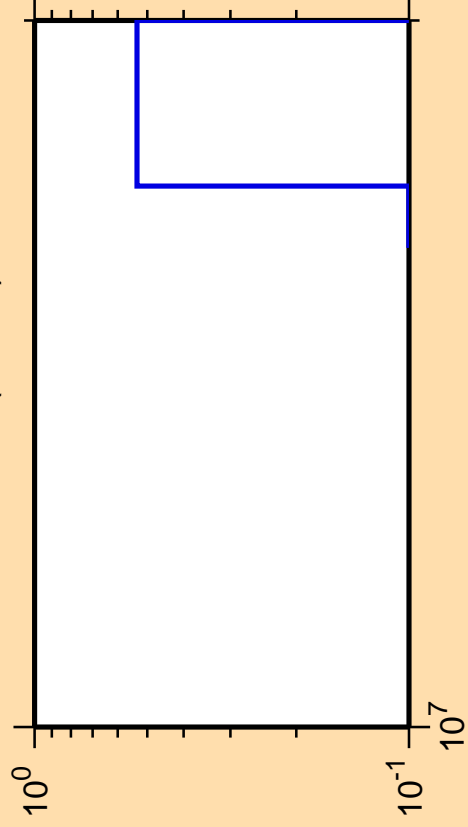
\Delta\sigma/\sigma vs. E for ^{136}\text{La} (mt 34)
