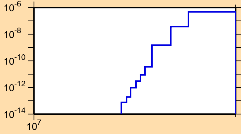
\sigma vs. E for ^{136}\text{La}(n,2n\alpha)
