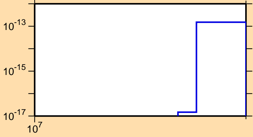
\sigma vs. E for ^{136}\text{La}(n,pd)
