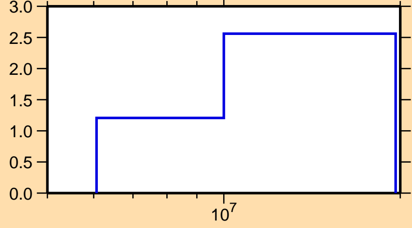
\Delta\sigma/\sigma vs. E for ^{136}\text{La}(n,\text{tot.})
