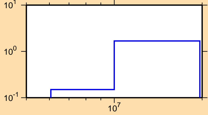
\sigma vs. E for ^{136}\text{La}(n,2n)
