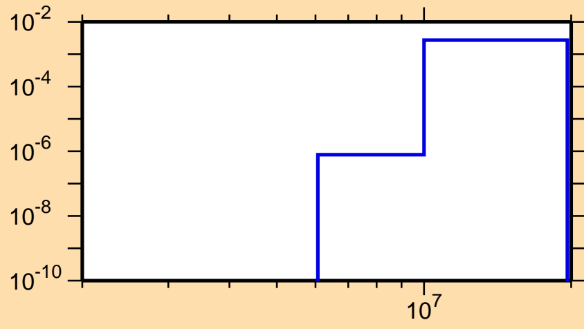
\sigma vs. E for ^{136}\text{La}(n,d)
