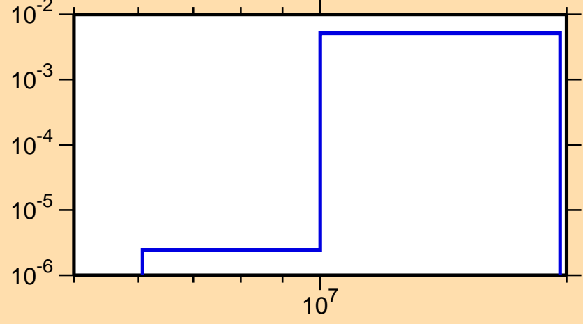
\sigma vs. E for ^{136}\text{La}(n,np)
