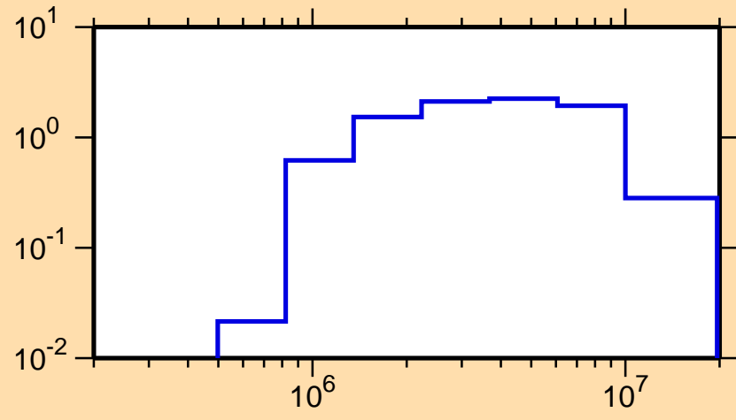
\sigma vs. E for ^{136}\text{La}(n,n\text{cont.})
