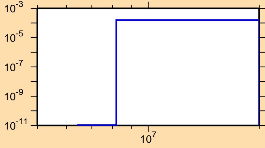
\sigma vs. E for ^{136}\text{La}(n,t)
