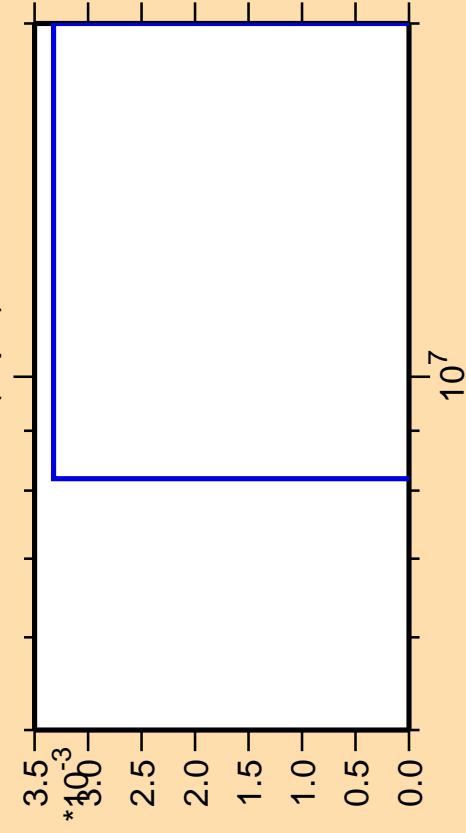
\Delta\sigma/\sigma vs. E for ^{136}\text{La}(n,pd)
