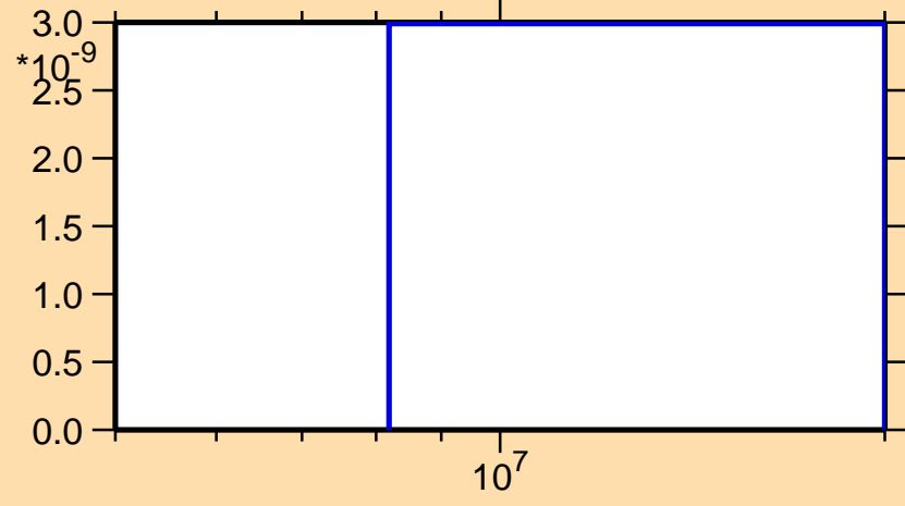
\sigma vs. E for ^{136}\text{La}(n,\text{He3})
