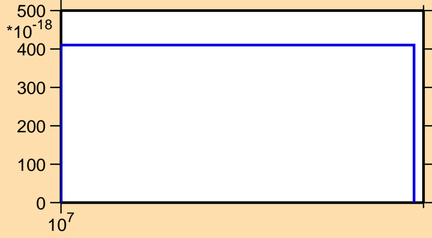
\sigma vs. E for ^{137}\text{La} (mt 45)
