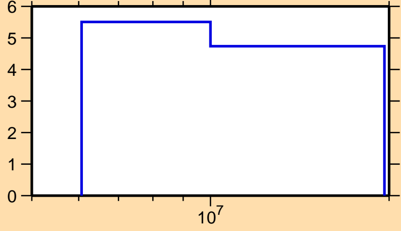
\Delta\sigma/\sigma vs. E for ^{137}\text{La}(n,\text{nonel.})
