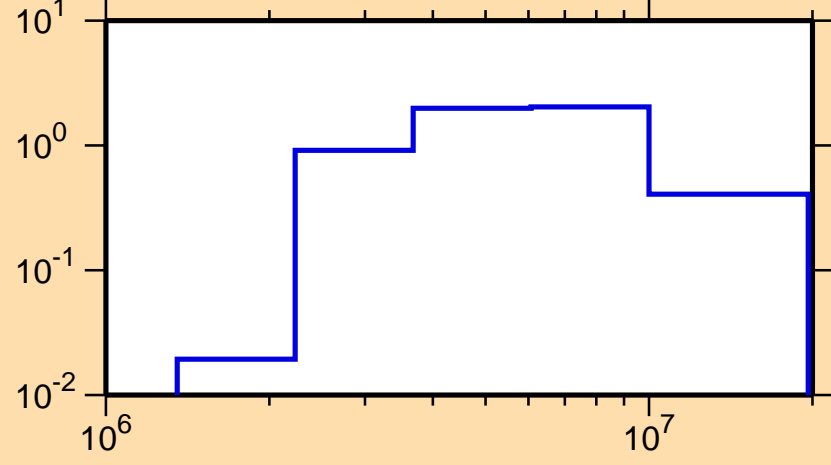
\sigma vs. E for ^{137}\text{La}(n,n\text{cont.})
