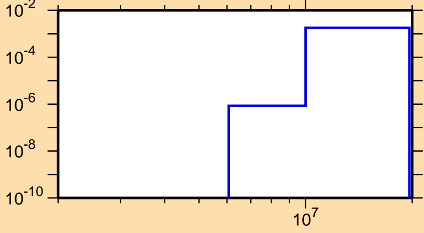
\sigma vs. E for ^{137}\text{La}(n,d)
