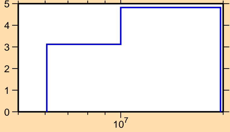
\Delta\sigma/\sigma vs. E for ^{137}\text{La}(n,\text{tot.})
