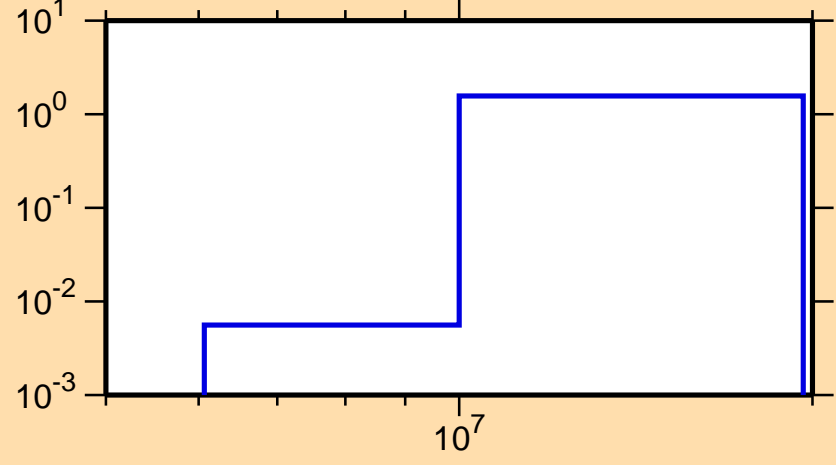
\sigma vs. E for ^{137}\text{La}(n,2n)
