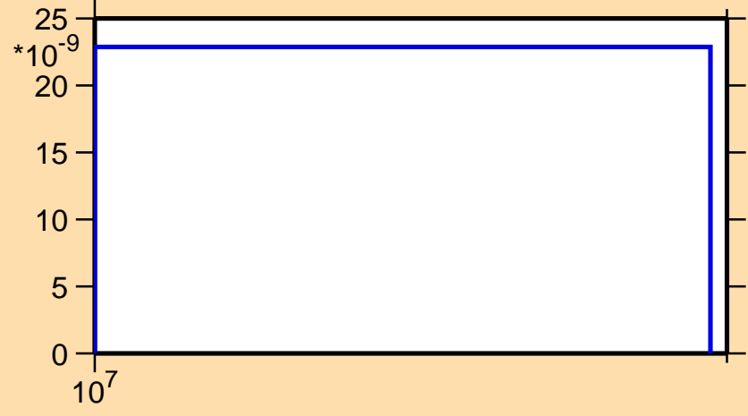
\sigma vs. E for ^{137}\text{La}(n,\text{nd})
