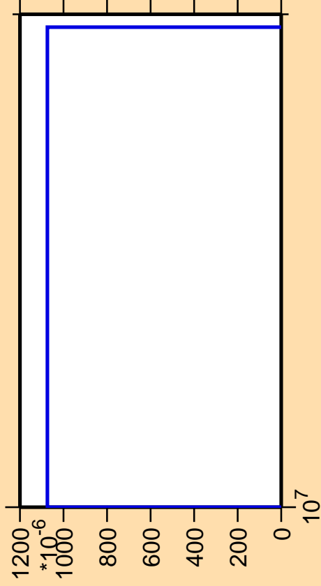
\Delta\sigma/\sigma vs. E for ^{137}\text{La} (mt 45)
