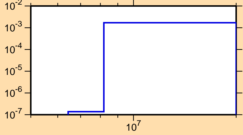
\sigma vs. E for ^{137}\text{La}(n,np)
