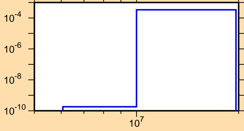
\sigma vs. E for ^{138}\text{La}(n,t)
