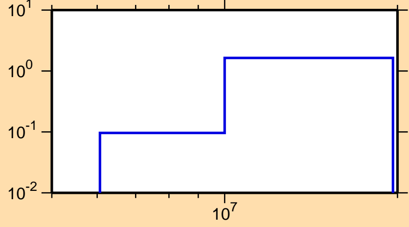
\sigma vs. E for ^{138}\text{La}(n,2n)
