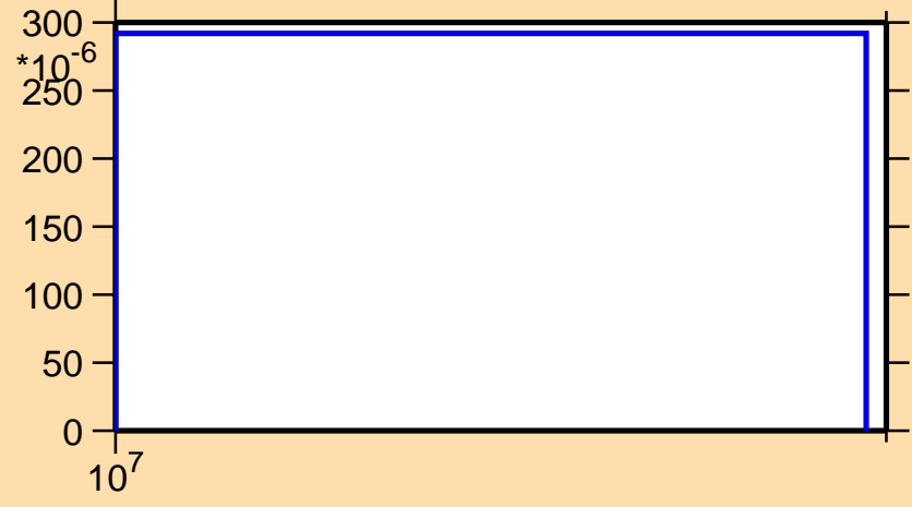
\sigma vs. E for ^{138}\text{La}(n,3n)
