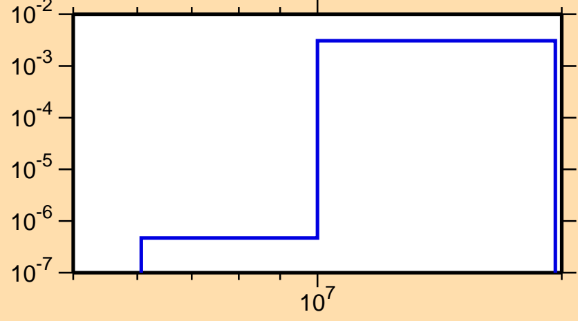
\sigma vs. E for ^{138}\text{La}(n,d)
