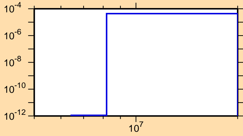
\sigma vs. E for ^{138}\text{La}(n,n\alpha)
