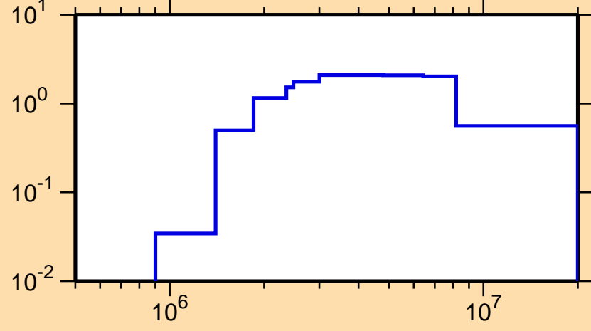
\sigma vs. E for ^{138}\text{La}(n,n\text{cont.})
