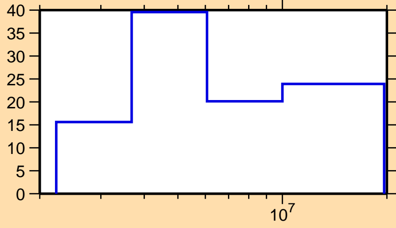
\Delta\sigma/\sigma vs. E for ^{139}\text{La}(n,p)
