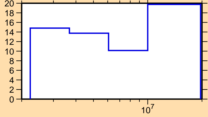
\Delta\sigma/\sigma vs. E for ^{139}\text{La}(n,ncont.)
