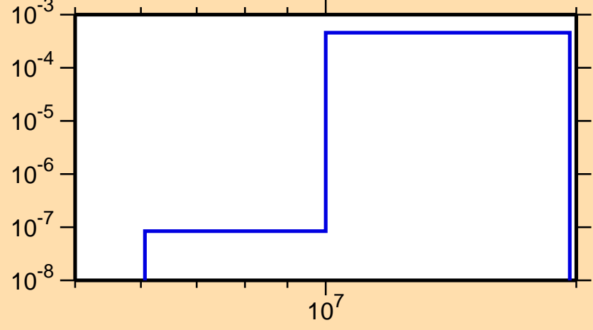
\sigma vs. E for ^{139}\text{La}(n,np)
