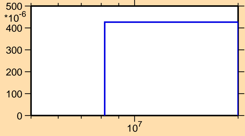
\sigma vs. E for ^{139}\text{La}(n,3n)
