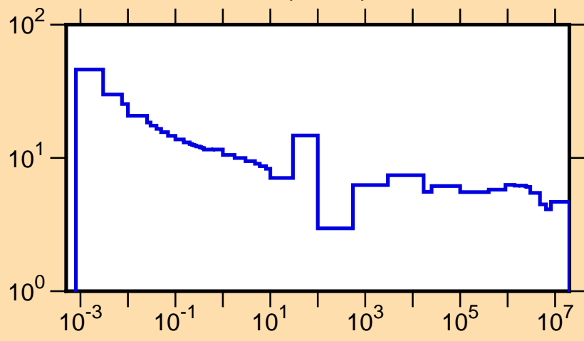
\sigma vs. E for ^{139}\text{La}(n,\text{tot.})
