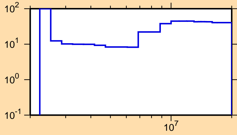
\Delta\sigma/\sigma vs. E for ^{141}\text{La}(n,n\text{cont.})
