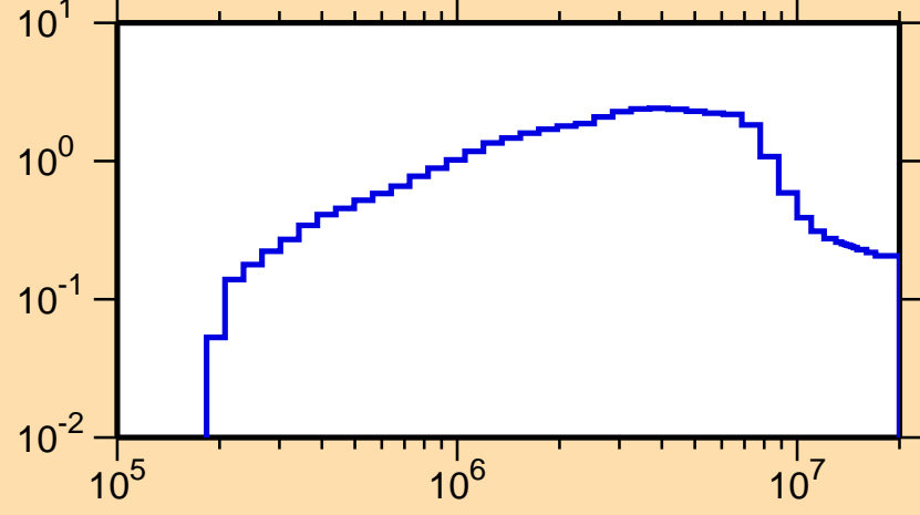
\sigma vs. E for ^{141}\text{La}(n,\text{inel.})
