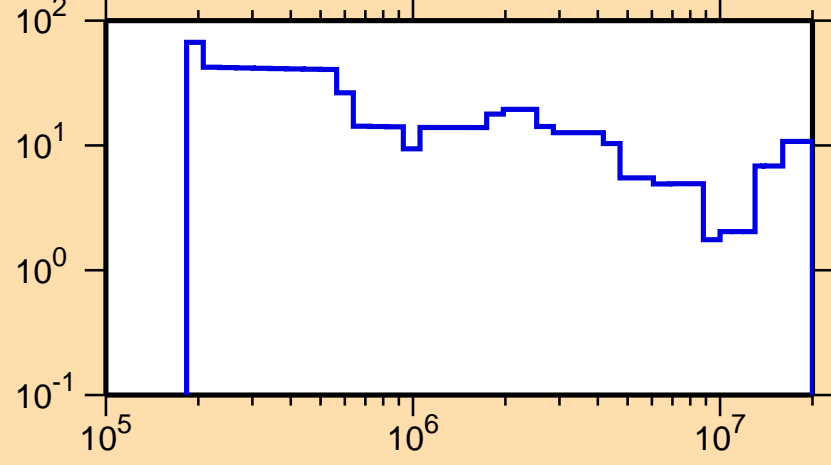
\Delta\sigma/\sigma vs. E for ^{141}\text{La}(n,\text{tot.})
