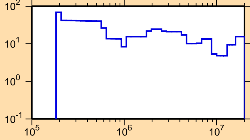
\Delta\sigma/\sigma vs. E for ^{141}\text{La}(n,\text{el.})
