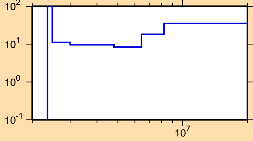
\Delta\sigma/\sigma vs. E for ^{141}\text{La}(n,n_{\text{cont}})
