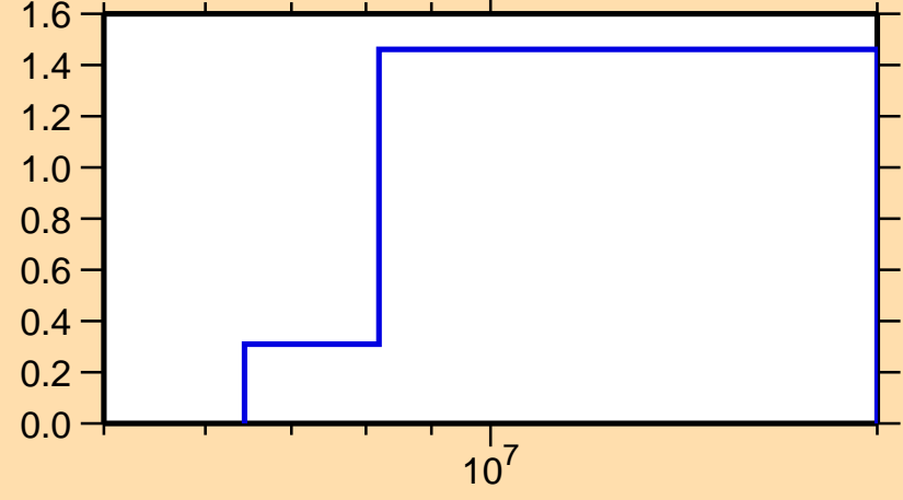
\sigma vs. E for ^{141}\text{La}(n,2n)
