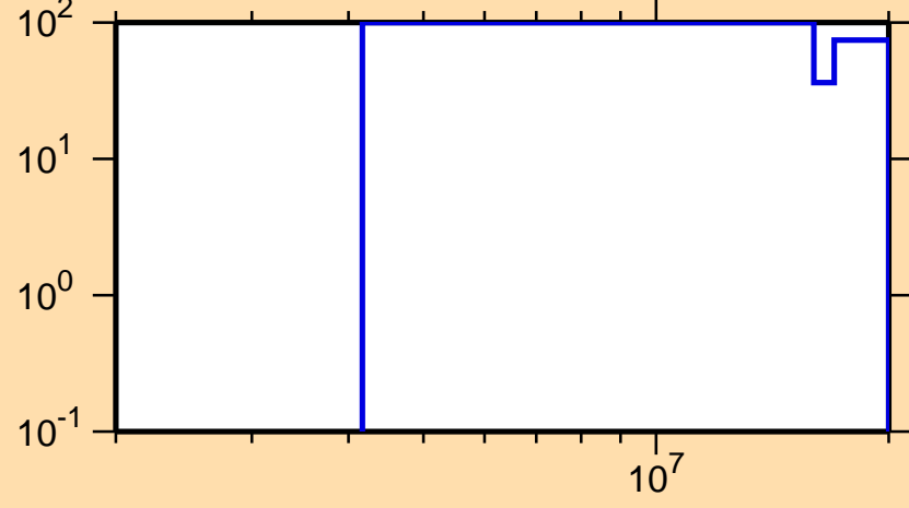
\Delta\sigma/\sigma vs. E for ^{143}\text{La}(n,n_1)
