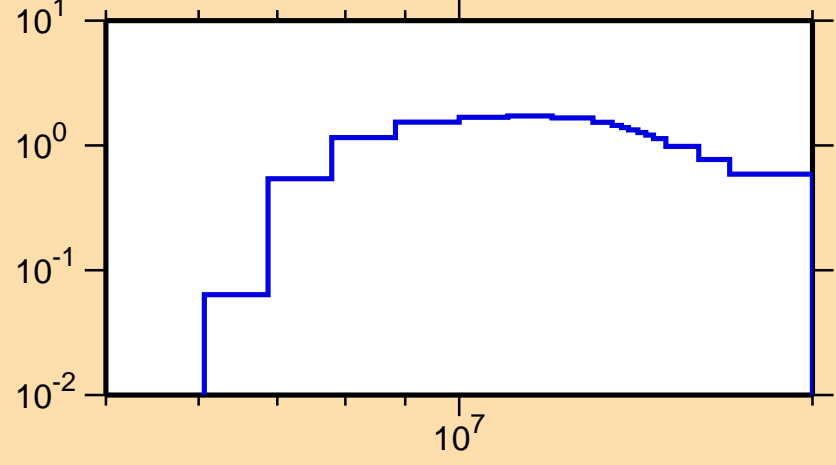
\sigma vs. E for ^{143}\text{La}(n,2n)
