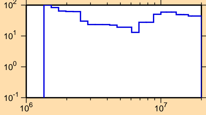
\Delta\sigma/\sigma vs. E for ^{143}\text{La}(n,n\text{cont.})
