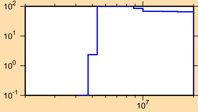
\Delta\sigma/\sigma vs. E for ^{143}\text{La}(n,p)
