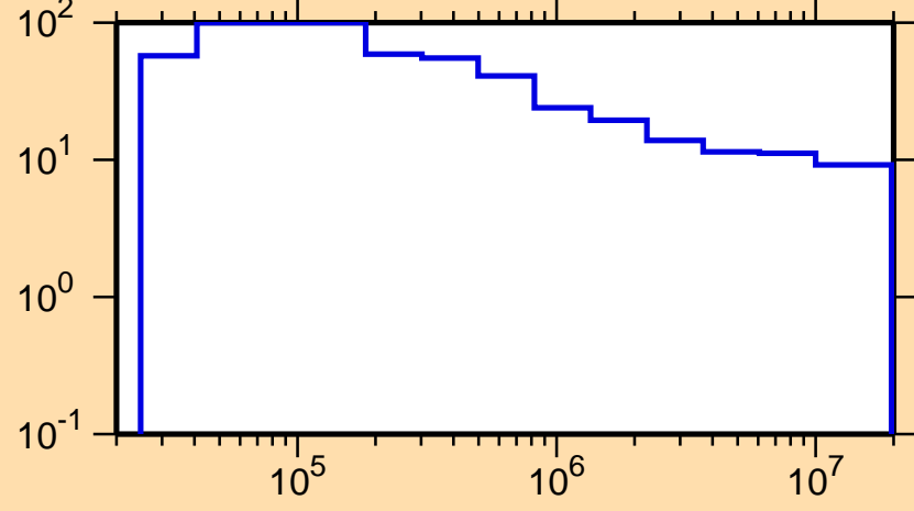
\Delta\sigma/\sigma vs. E for ^{143}\text{La}(n,\text{nonel.})
