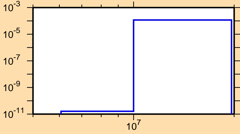
\sigma vs. E for ^{143}\text{La}(n,t)
