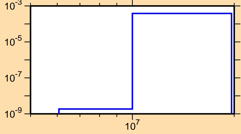
\sigma vs. E for ^{143}\text{La}(n,d)
