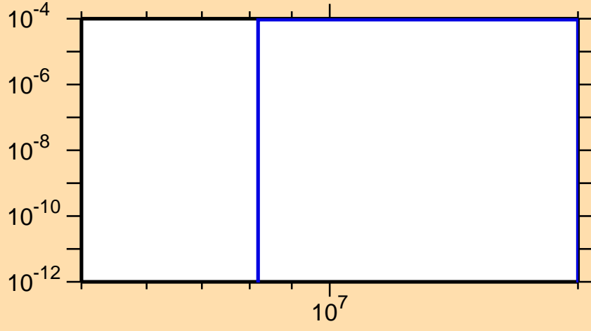
\sigma vs. E for ^{143}\text{La}(n,t)
