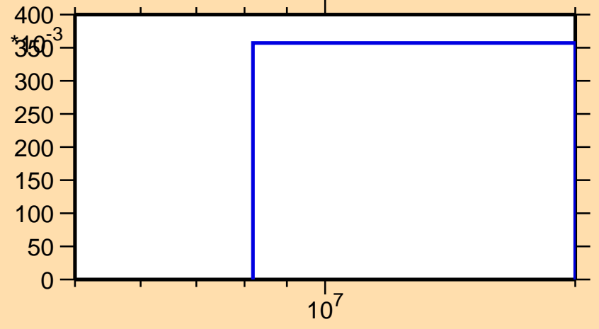
\sigma vs. E for ^{143}\text{La}(n,3n)
