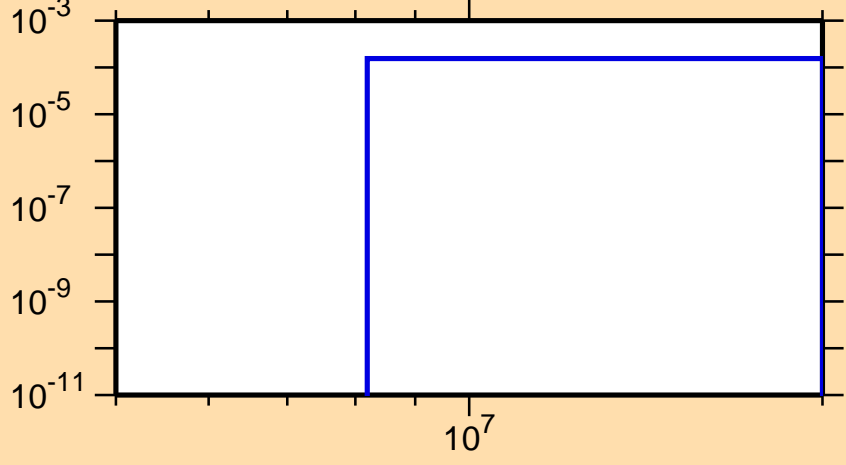
\sigma vs. E for ^{143}\text{La}(n,np)
